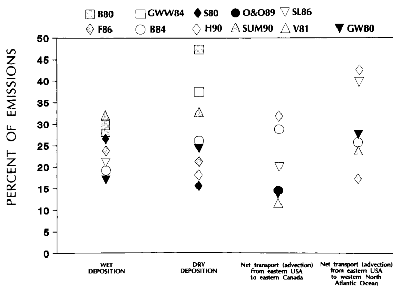
Fig. 4. Fluxes of sulfur in the atmosphere of the eastern US expressed as percent of emissions. The solid and open symbols indicate that the budgets were products of data analysis or models, respectively (Galloway and Rodhe, 1991). Reproduced by permission of the Royal Society of Edinburgh.
