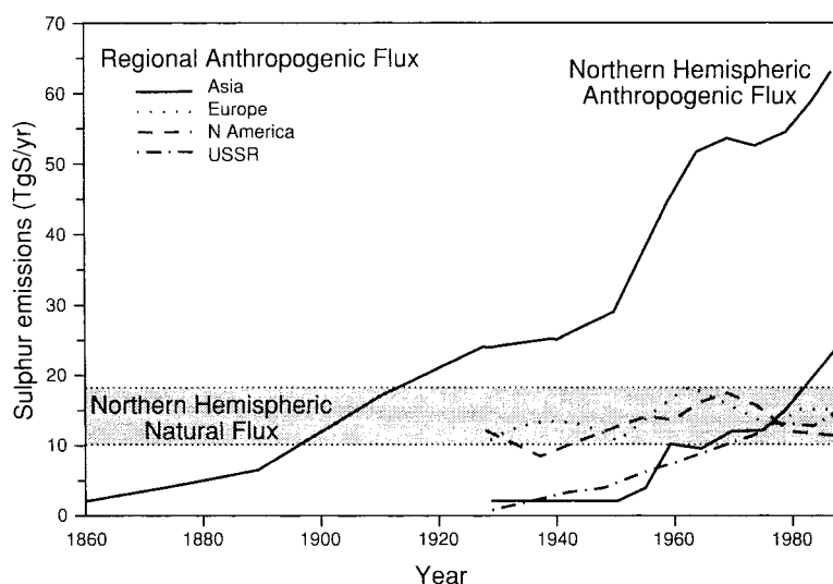
Fig. 2. The evolution of northern hemisphere and regional man-made sulfur emissions since 1860 (Dignon and Hameed, 1989; IPCC, 1996). Reproduced by permission of IPCC.
