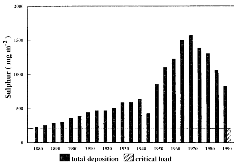
Fig. 3. Calculated historical trends of sulfur deposition in southern Sweden (Mylona, 1996).
