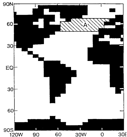
Fig. 2. Region A indicates the area where freshwater is discharged in the freshwater integration (from MS97).
