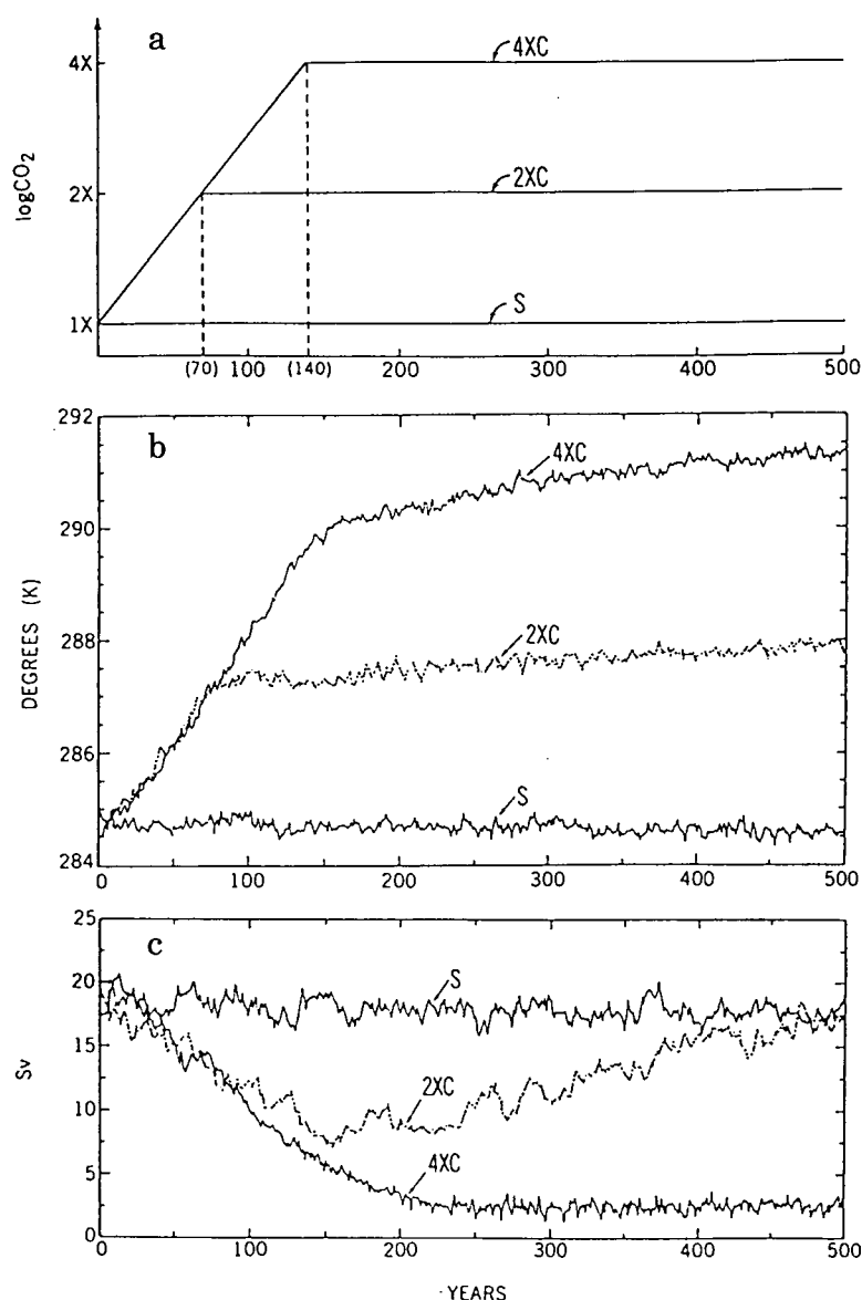
Fig. 12. Temporal variations of: (a) logarithm of atmospheric \text{CO}_2 concentration; (b) global mean surface air temperature (K); (c) the intensity of the THC in the north Atlantic; obtained from 4 \times \text{C} , 2 \times \text{C} and \text{S} (from MS94). Here, the intensity of the THC is defined as the maximum value ( \text{Sv} ) of the streamfunction representing the meridional overturning in the North Atlantic Ocean.
