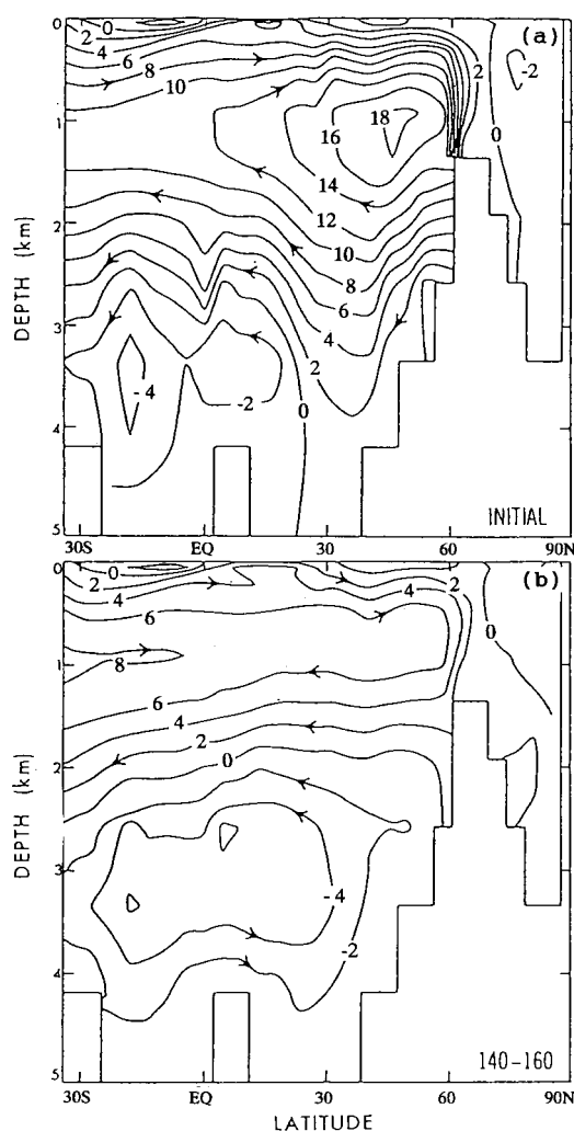
Fig. 14. Streamfunction of meridional circulation (Sv) in the Atlantic Ocean from the 2 \times C . (a) Initial condition. (b) Average over the 140th–160th year (from MS94).
