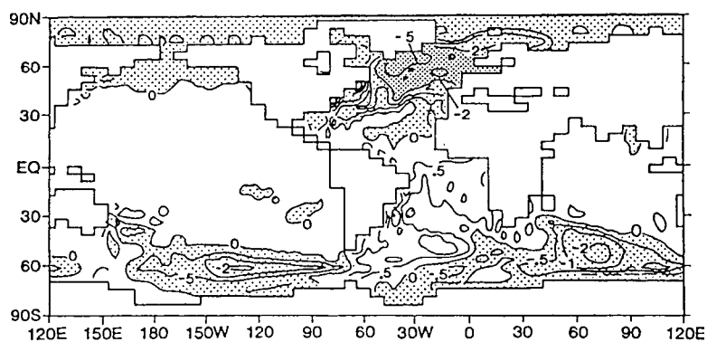
Fig. 6. Geographical distribution of SST anomalies (°C) averaged over year 401–500 of the freshwater integration. The anomalies are defined as the difference between the freshwater and the control integrations (from MS97). The logarithmic contouring is employed with contour values of 0.5, 1, 2 and 5.
