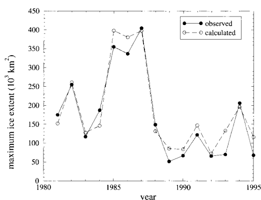
Fig. 5. Observed and calculated annual maximum ice extent for the Baltic Sea.
