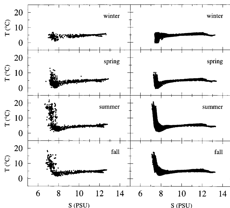
Fig. 4. Seasonal T - S diagrams based on observations (left panels) and calculations (right panels) from the Eastern Gotland Basin. The observations are from BY15.
