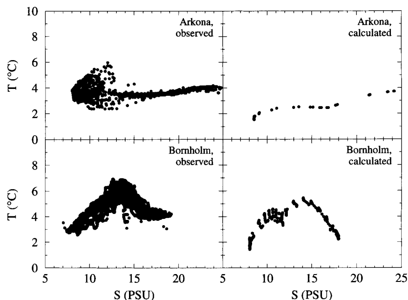
Fig. 8. Observed (left panels) and numerically simulated (right panels) temperature and salinity structures for the Arkona Basin (top panels), from 6–8 February 1993, and the Bornholm Basin (bottom panels), from 1–31 March 1993, during the major Baltic inflow.
