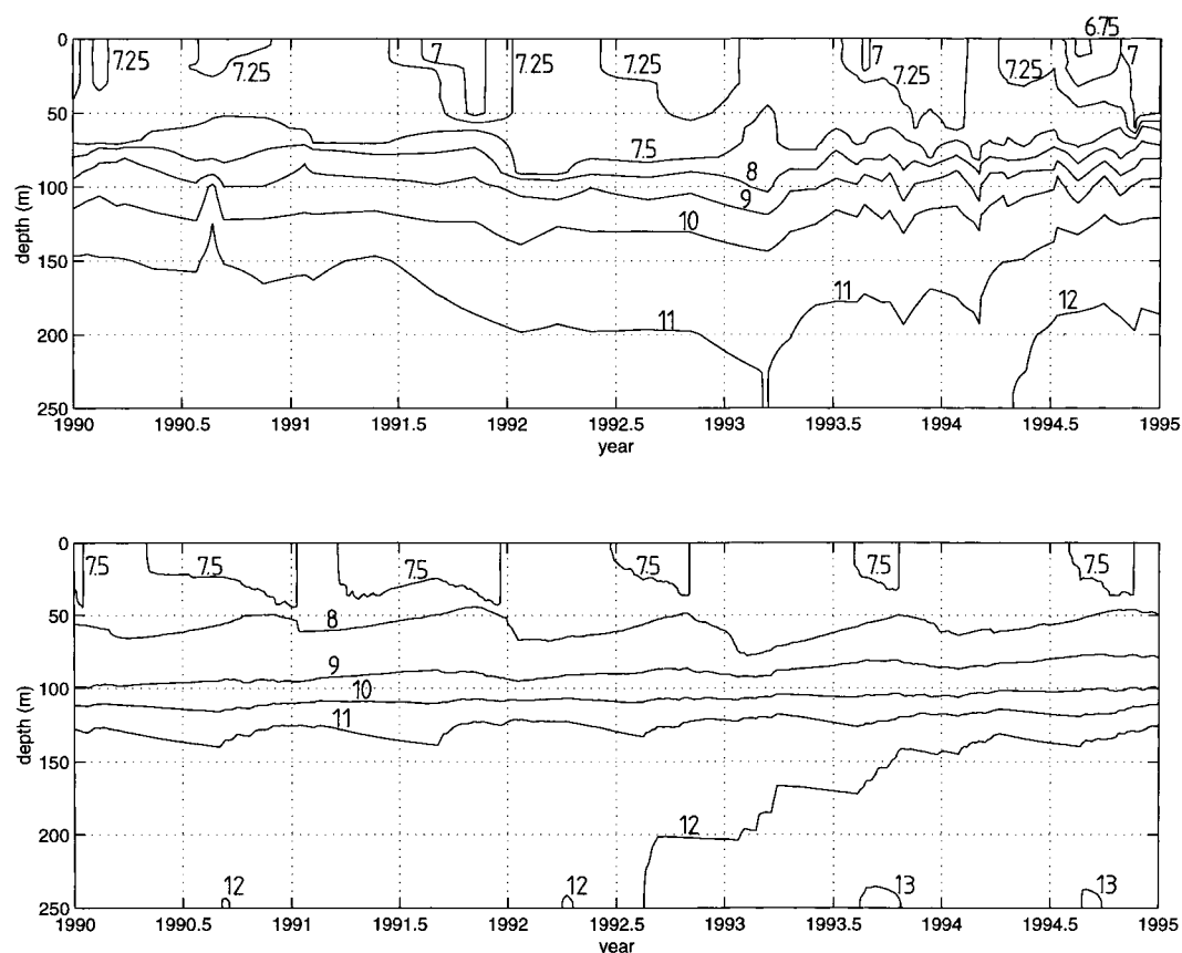
Fig. 7. Observed (top) and calculated (bottom) salinity fields (PSU) in the Eastern Gotland Basin for the period 1990–1995.
