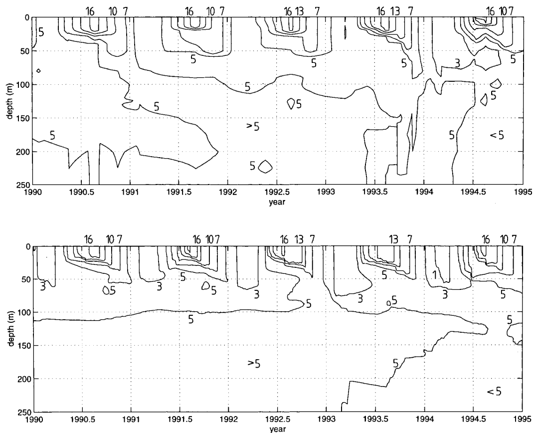
Fig. 6. Observed (top) and calculated (bottom) temperature fields ( ^{\circ}\text{C} ) in the Eastern Gotland Basin for the period 1990–1995.
