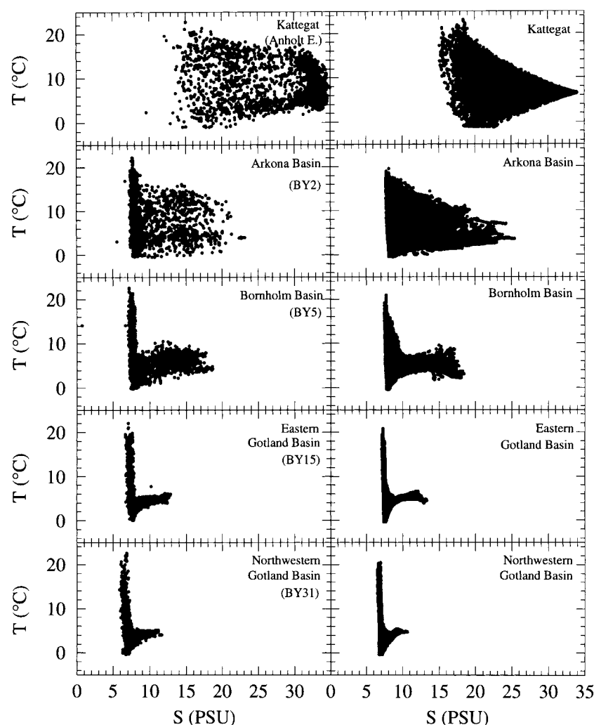
Fig. 3. T - S diagrams based on observations (left panels) and calculations (right panels) from the Kattegat, the Arkona Basin, the Bornholm Basin, the Eastern Gotland Basin, and the Northwestern Gotland Basin.
