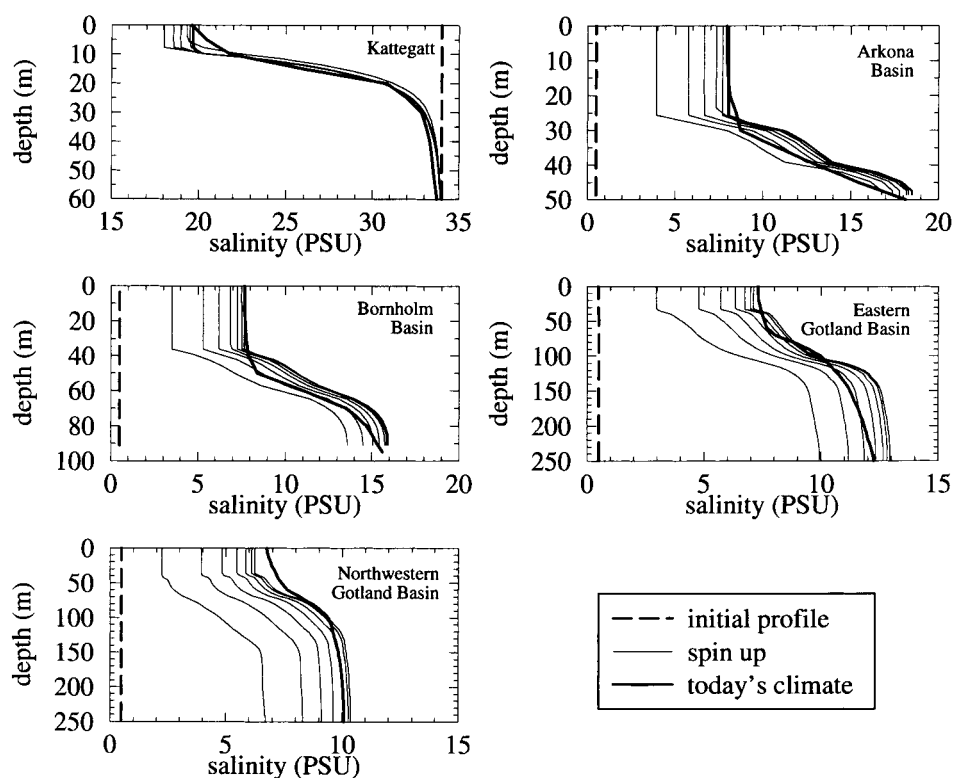
Fig. 9. An illustration of a 105-year stratification spin-up in the Kattegat, the Arkona Basin, the Bornholm Basin, the Eastern Gotland Basin, and the Northwestern Gotland Basin. The initial profiles are dashed, the results from the spin-up are shown as thin lines with 15-year intervals, and the observed median profiles are shown as thick lines.
