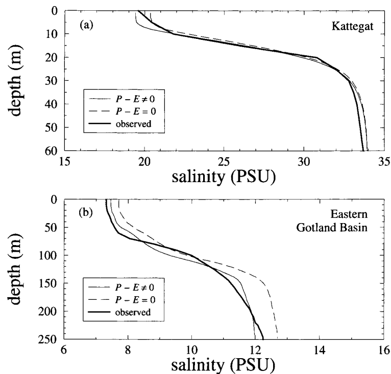
Fig. 10. Median salinities for the Kattegat (a) and the Eastern Gotland Basin (b) from 15-year calculations (1980–1995), with and without the meteorological runoff (precipitation minus evaporation, P-E ).
