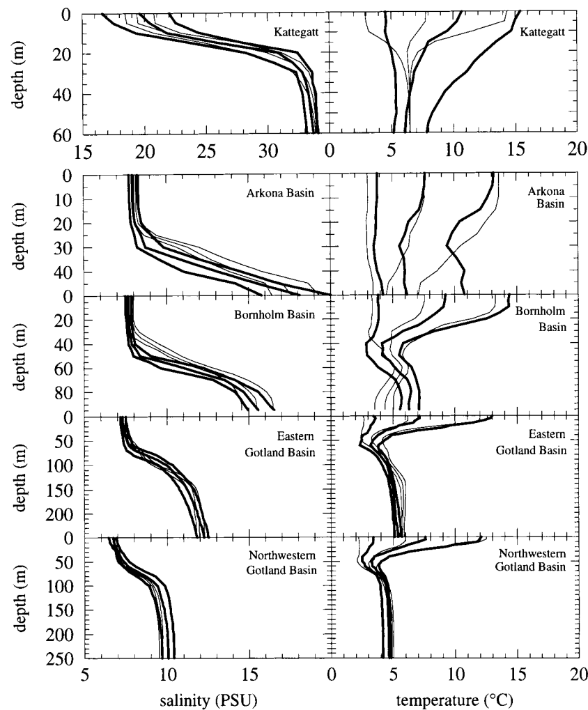
Fig. 2. Median profiles of salinity (left panels) and temperature (right panels) from the Kattegat, the Arkona Basin, the Bornholm Basin, the Eastern Gotland Basin, and the Northwestern Gotland Basin, based on observations (thick lines) and calculations (thin lines) from 1 November 1980 to 1 November 1995. The curves represent the 3 quartiles, the middle ones being the medians.
