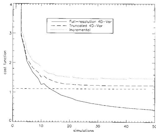
Fig. 13. Variation of the cost function with the number of simulations obtained for the full-resolution 4D-Var (solid line), the truncated 4D-Var (long dashes) and incremental 4D-Var (dotted) when random noise are added to the observations in the low-resolution observation network. The short dashed line indicates the total variance of the random noise.
