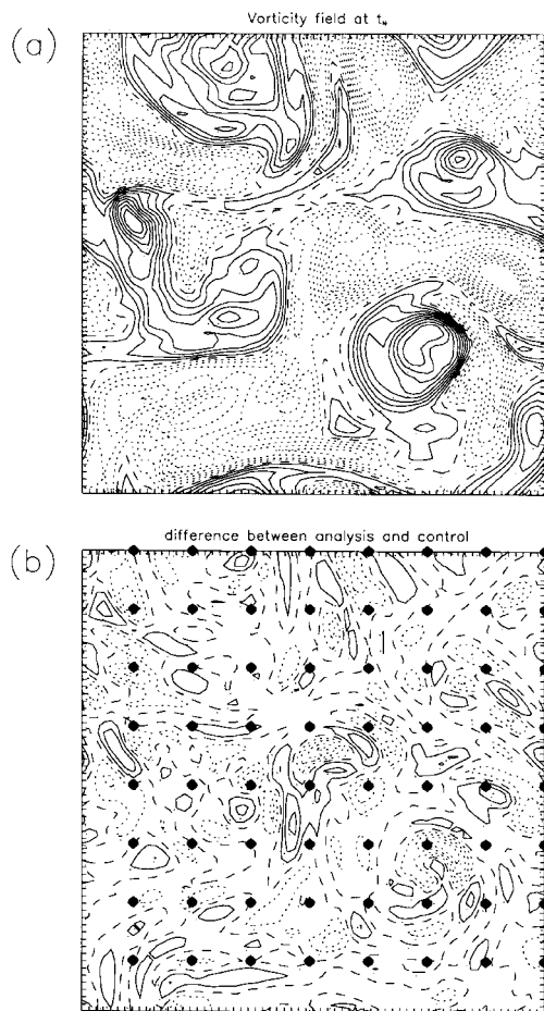
Fig. 14. (a) Vorticity field at the end of the assimilation period obtained with the full-resolution 4D-Var formulation after 20 simulations when random noise is added to the observations in the low-resolution observation network. (b) Difference between (a) and the control run vorticity field. The large dots indicate the position of the observations.
