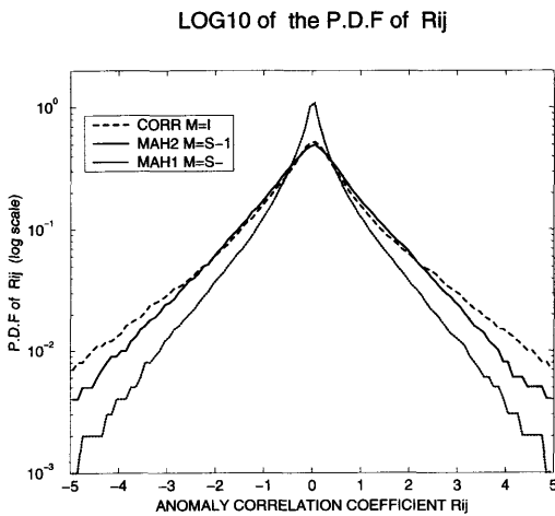
Fig. 3. The probability distributions of the anomaly correlation coefficient R_{kl} = z_k^T \mathbf{M} z_l (logarithmic scale) for 3 different metrics. The bin size was chosen to be 0.1 and no smoothing has been applied.
