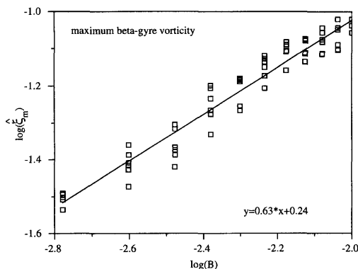
Fig. 9. The non-dimensional maximum beta gyre vorticity \hat{\xi}_m is plotted against the non-dimensional beta parameter. Several points from each of eleven simulations are shown. A log-log plot is used to reveal power law relationships. The solid line is eq. (29).
