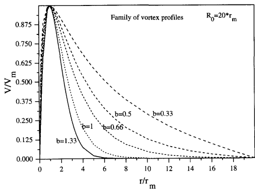
Fig. 1. The family of vortex profiles used in this investigation. The ratio of wind speed to the maximum wind speed ( V_m ) is plotted against the ratio of radius to the radius of maximum wind ( r_m ).
