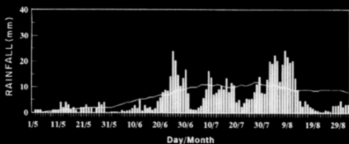
Fig. 2. Histogram of areal mean daily precipitation ( \text{mm day}^{-1} ) over the trough area except for the blocks close to the foothills of Himalayas between 25^\circ – 27.5^\circ N and 80^\circ – 90^\circ E. The solid curve across the histogram represents long term (1901–1980) daily normal rainfall.
