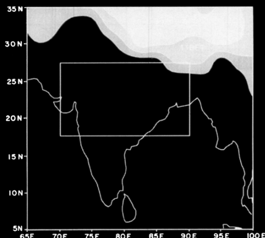
Fig. 1. ECMWF FGGE-Level III b data domain at 2.5^\circ \times 2.5^\circ grid interval used in the study. The rectangular box covers the domain of monsoon trough bounded by 17.5^\circ – 27.5^\circ N and 70^\circ – 90^\circ E. The shaded area represents the topography of 1500 m and above.
