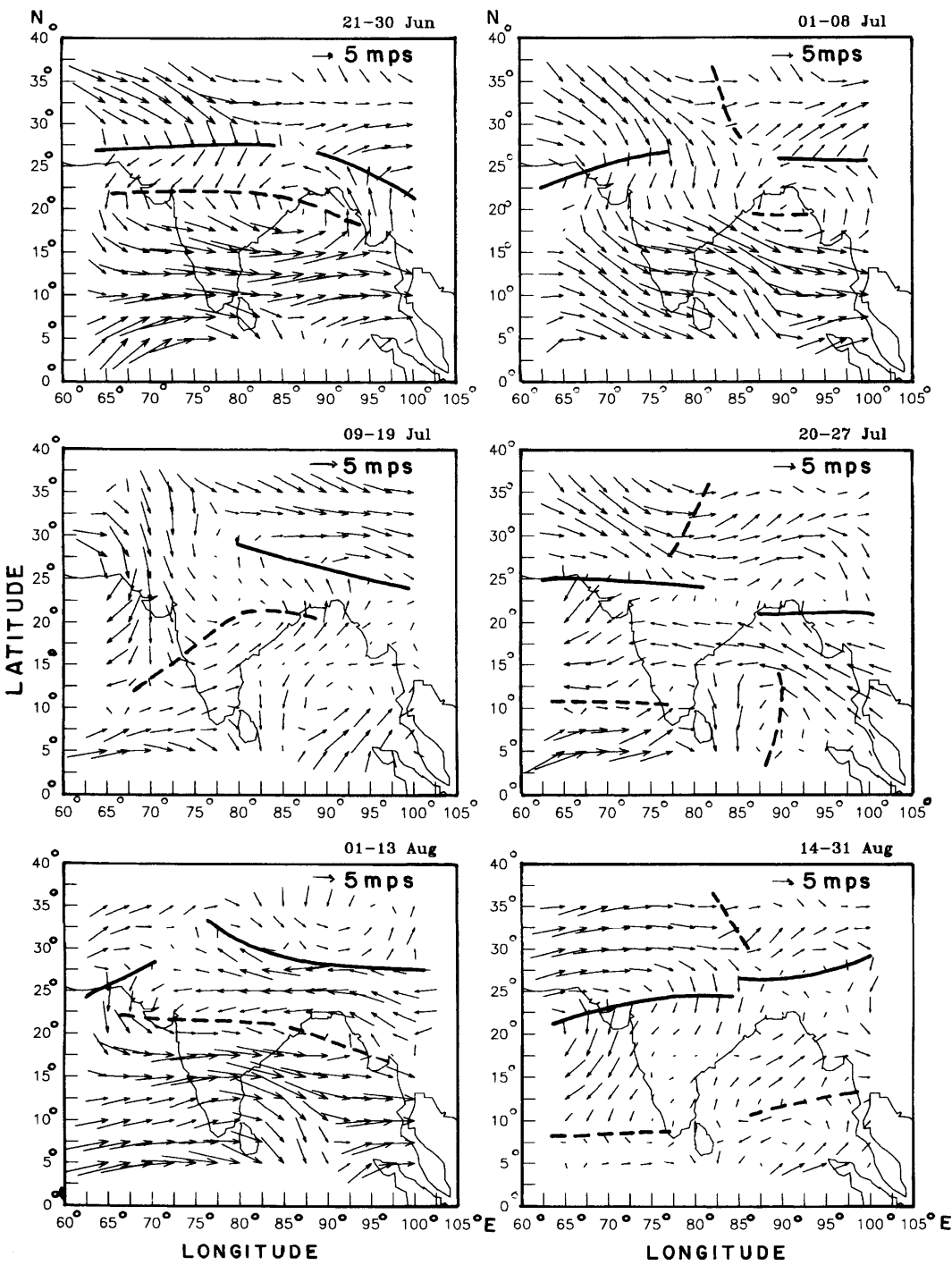
Fig. 4. ECMWF-FGGE Level IIIb mean winds at 500 hPa level for different phases of monsoon. The axis of the troughs and ridges are shown by dashed and solid lines respectively. (Unit vector arrow represents 5 mps).
