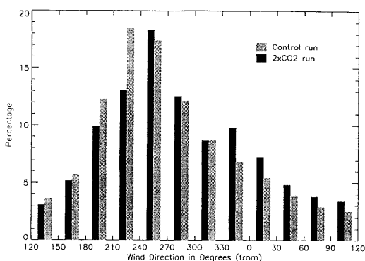
Fig. 4. Distribution of wind directions (DJF) for an area north of Scotland (60.0–64.5°N, 9.0°W–0.0°). Control experiment and 2\times\text{CO}_2 experiment.
