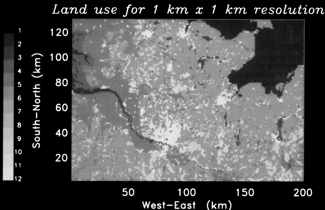
Fig. 2. Land-use data set for the inner model domain with a 1 \times 1 \text{ km}^2 resolution (after Mölders and Raabe, 1996). The numbers represent the land-use types as follows: 1 water deeper than 10 m, 2 water less than 10 m deep, 3 lake/river, 4 sand, 5 grassland, 6 agriculture, 7 heather/bushland, 8 deciduous forest, 9 mixed forest, 10 coniferous forest, 11 village, and 12 town.
