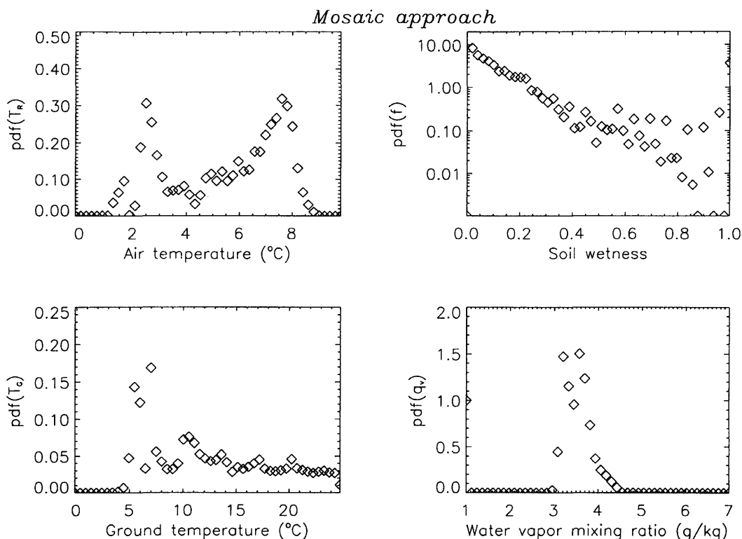
Fig. 4. Probability density functions, pdf, from upper left to lower right corner for air temperatures, T_R , at reference height (in 10 m), soil wetness factor, f , ground temperatures, T_G , and water vapor, q_v , at reference height for the simulation using the mosaic approach.
