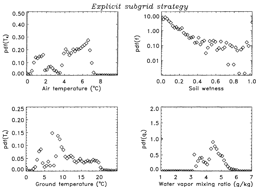
Fig. 5. As Fig. 4 but for the simulation with the explicit subgrid strategy.
