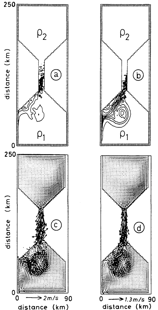
Fig. 6. Density and current fields in layers 1 and 5 (a-d). Maximum velocities are 1.66 m/s and 1.30 m/s for c and d, respectively.
