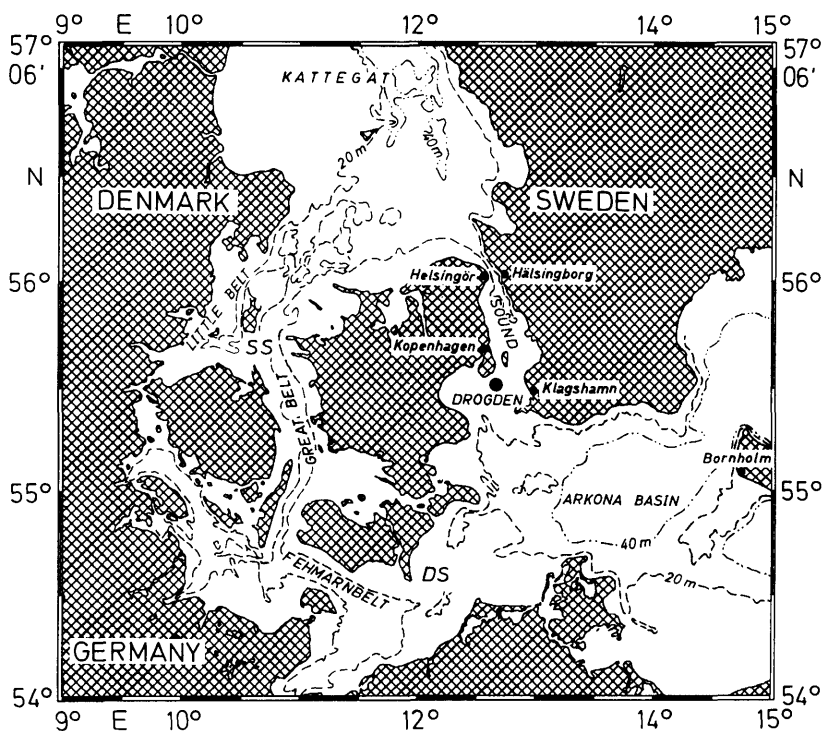
Fig. 1. The Danish Straits, Kattegat and Arkona Basin. SS = Samsø Sill. DS = Dars Sill. The Belt Sea is the area between Kattegat and Arkona basin.
