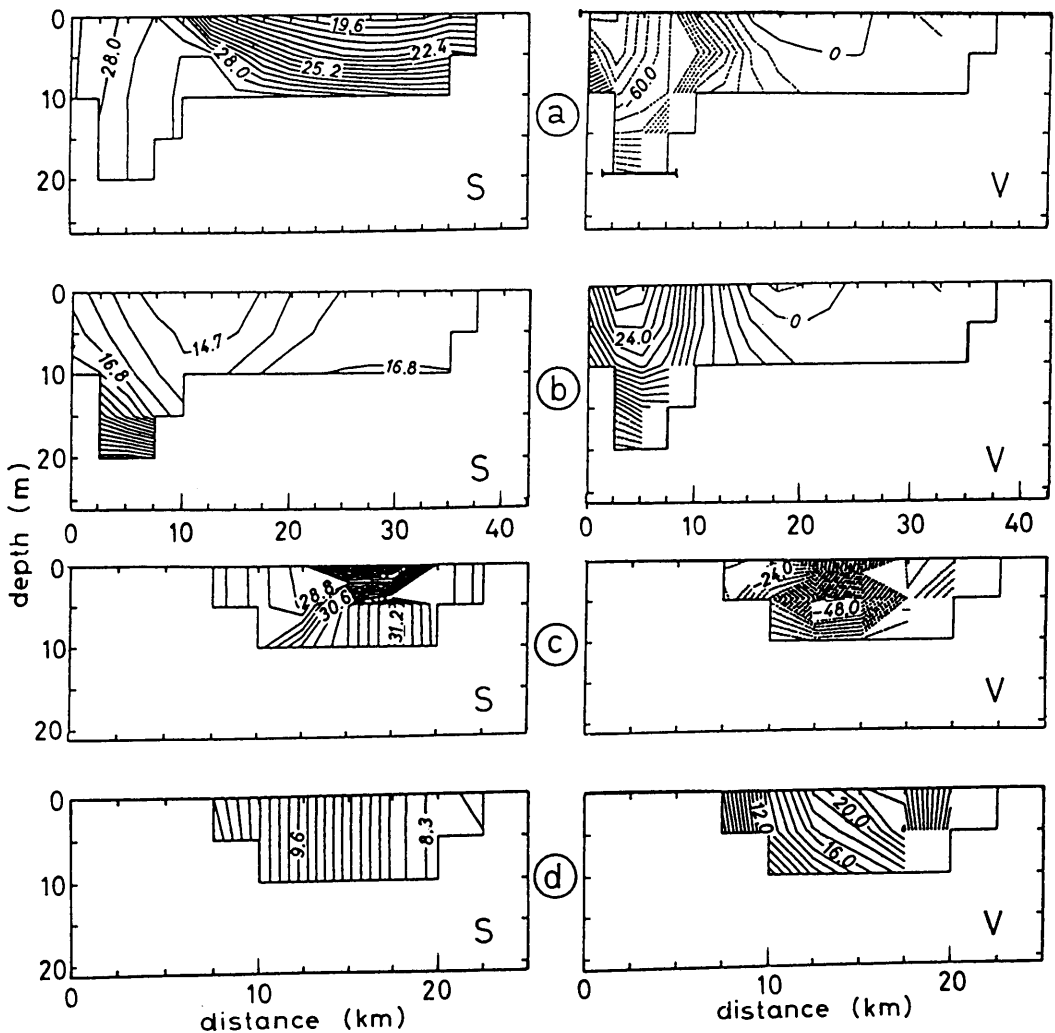
Fig. 14. Salinity and current distributions (currents in 10^{-2} m/s). (a) Inflow and (b) outflow in the Great Belt. (c) Inflow and (d) outflow in the Sound.
