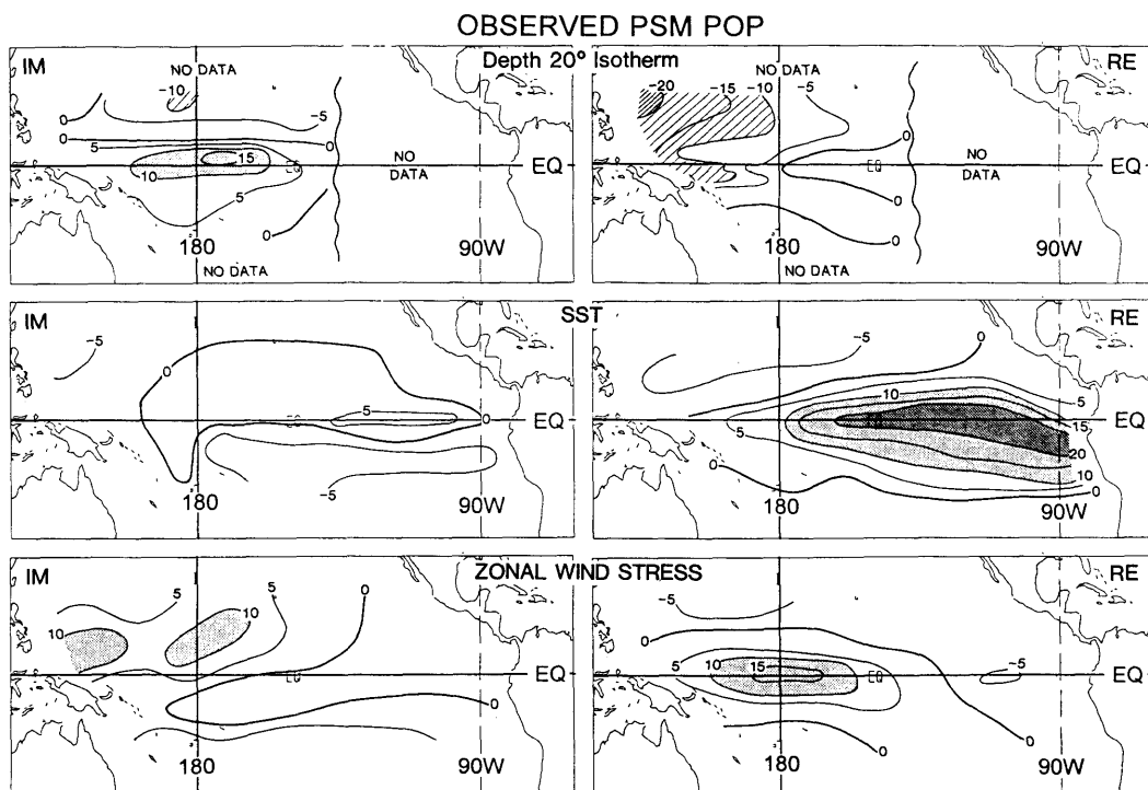
Fig. 2. Spatial patterns of the PSM POP. Left: imaginary part patterns. Right: real part patterns. Upper: depth of 20°C isotherm, a surrogate for sea level. Middle: sea surface temperature. Lower: zonal wind stress.
