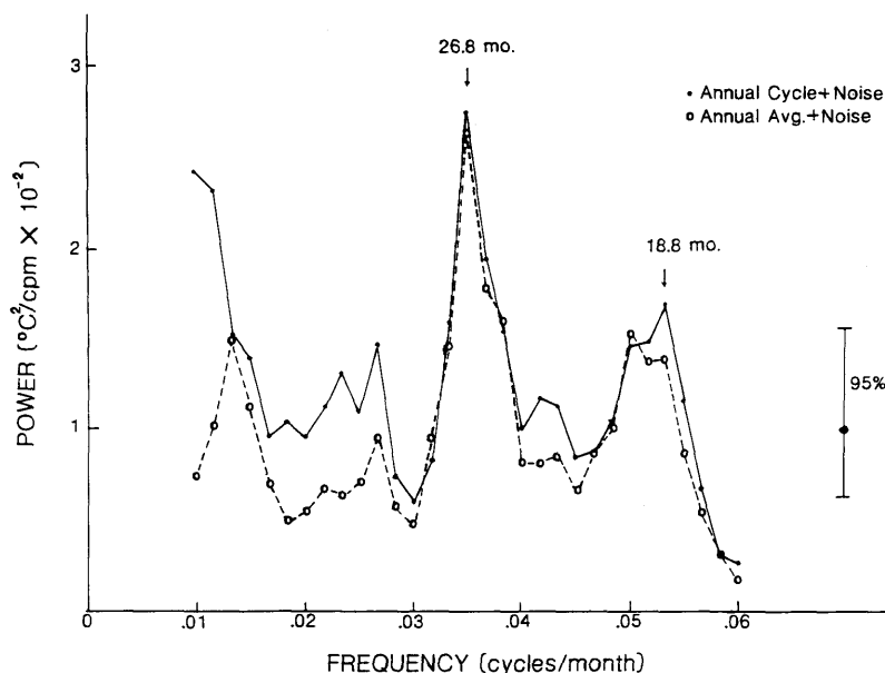
Fig. 4. Power spectra of NINO3 SST anomaly from 50-year OGCM runs forced by spatially red and temporally white anomalous wind stress. One run also included the regular seasonal cycle of wind stress (solid dot), while the other used annual average stress as climatological forcing (open circle). The NINO3 region is between 90–150°W and 5°N–5°S.
