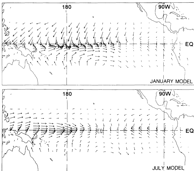
Fig. 8. Anomalous wind stress field produced by an observed warm SST anomaly (February 1992) from the atmospheric component of the HCM: upper, using January coefficients; lower, using July coefficients.
