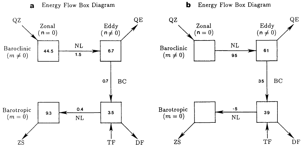
Fig. 3. Energy flow box diagram within zonal and eddy energies decomposed in barotropic and baroclinic components. (a) FGGE observation, (b) unstable Charney mode for n=6 . Units are 10^5 \text{ J m}^{-2} for energy and \text{W m}^{-2} for energy conversions. Percentile contributions are substituted for (b).
