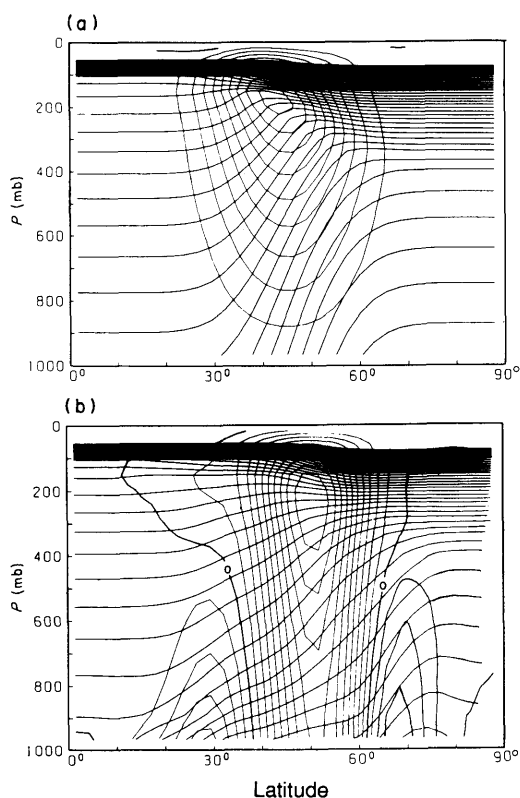
Fig. 1. Latitude-height cross sections showing potential temperature and zonal velocity in a baroclinic wave life-cycle experiment. Shown in (a) is the basic state and (b) the zonal field at day 15. The counter interval is 5 m/s for zonal velocity and 5 K for potential temperature (after Hoskins, 1983).
