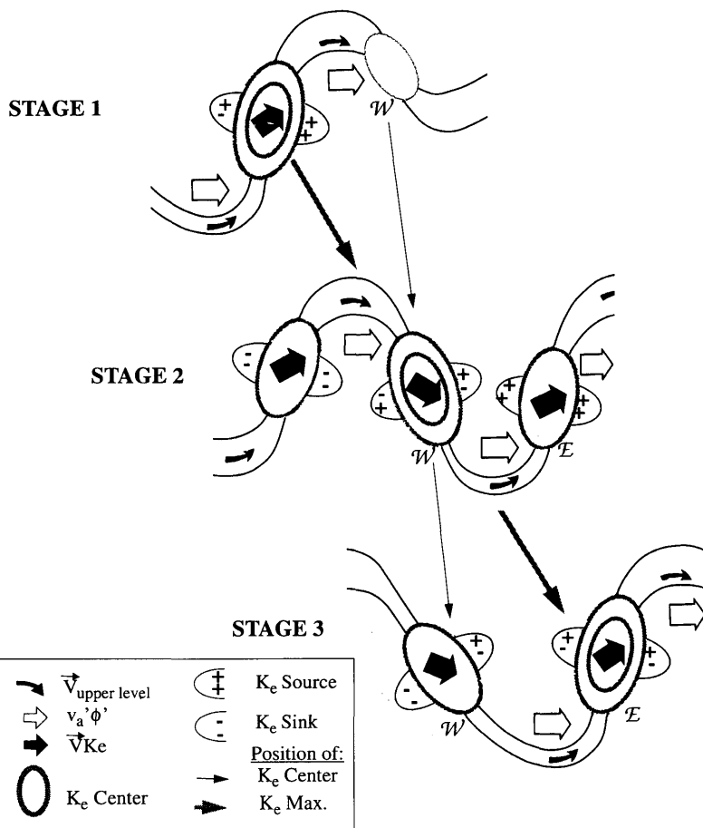
Fig. 3. The three stages in the evolution of a baroclinic wave. Symbols are as given in the figure. Stage 1 : Upstream system decay and generation of energy center W west of new trough via geopotential fluxes. Stage 2 : Energy fluxes emanate from a mature W and foster growth of energy center E east of trough. Stage 3 : Dissipation of energy center W , maturation of energy center E .
