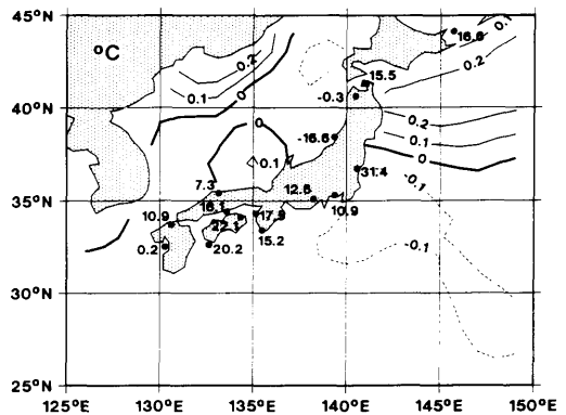
Fig. 7. 1st pair of canonical correlation patterns p_2^{sl} and q_2 of the joint analysis of Japanese sea level and regional sea-surface temperature. Units: mm and ^{\circ}\text{C} .
