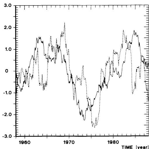
Fig. 10. Time coefficients \alpha_2(t) and z_2(t) of the second pair of canonical correlation patterns derived in the joint analysis of sea level (continuous line) and North Pacific sea-level pressure (dashed line). The time series are normalized to standard deviation 1.
