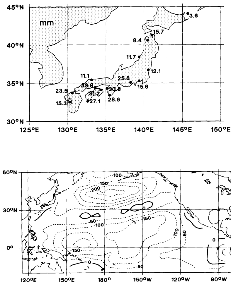
Fig. 14. 2nd pair of canonical correlation patterns p_2^{sl} and q_2 of the joint analysis of Japanese sea level and North Pacific sea-surface temperature. Units: K and mm.
