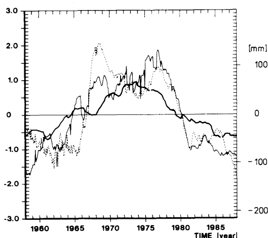
Fig. 9. Time coefficients \alpha_1(t) and z_1(t) of the first pair of canonical correlation patterns derived in the joint analysis of sea level (continuous line) and regional sea-surface temperature (dashed line). The time series are normalized to standard deviation 1. As heavy line the time-filtered sea level anomalies at Station 2 (for the location, see Fig. 8), at the northeast coast is shown for comparison.
