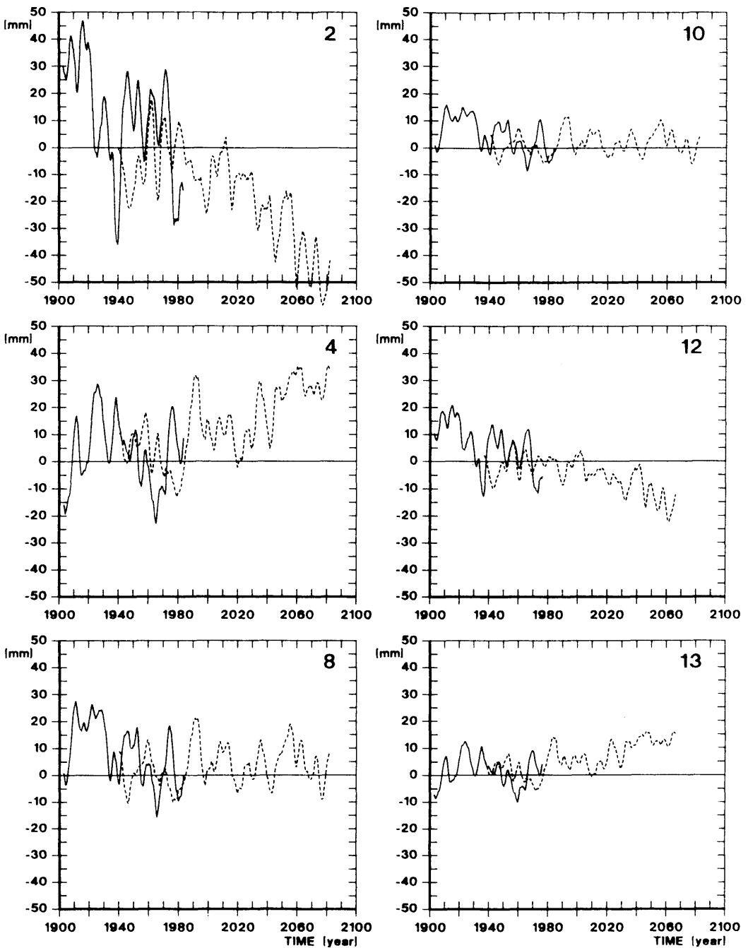
Fig. 15. Downscaled sea level changes at six Japanese tidal gauge sites as derived from observed sea-level pressure fields (continous line, from 1900 to 1988) and from simulated sea-level pressure anomalies (dashed line, from "1935" to "2085"). Only the sea-level component controlled by the anomalous large-scale circulation is taken care of by the downscaling procedure. Units: mm. For the station numbers see Fig. 1.
