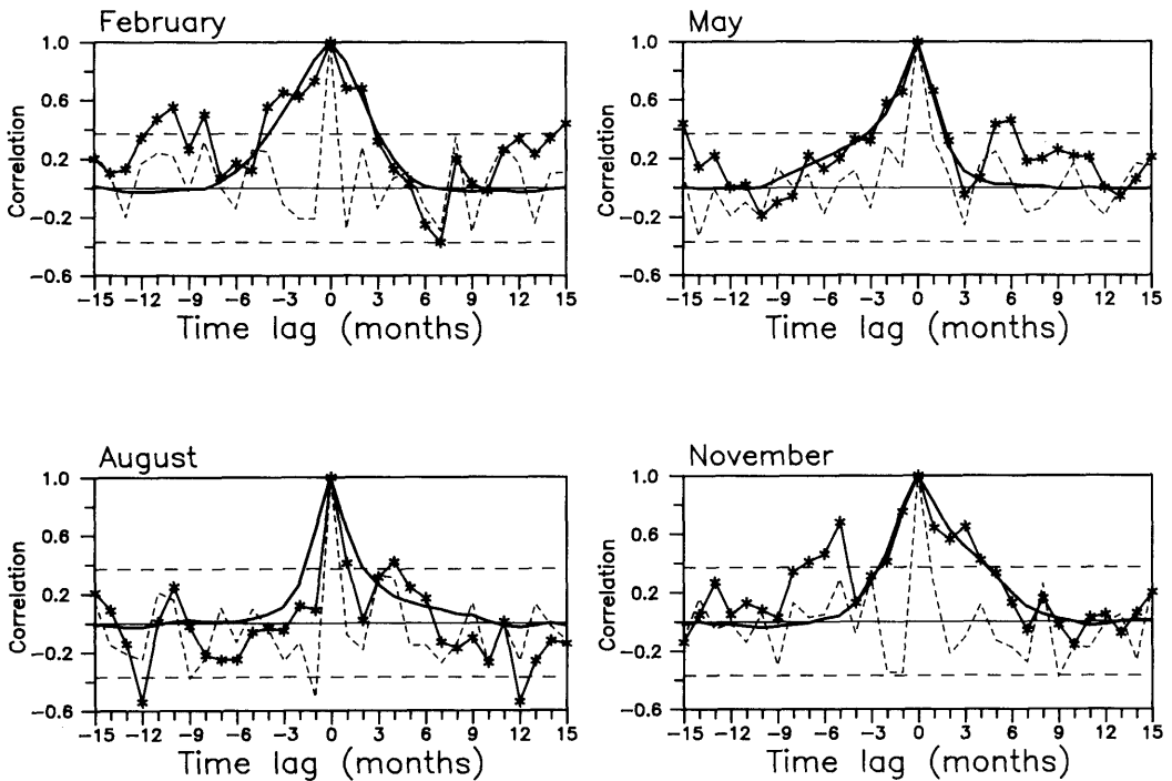
Fig. 1. Correlations of the data (full line with stars), Model II (full line) and forcing (dashed line), as functions of lag time at the grid point (175°W, 30°) for four seasons. Long dashed lines enclose the band where correlations are not significant at the 95% level.
