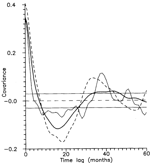
Fig. 2. Covariances of data (short dashed line), model III (full line) and an arbitrary realization of this model III as functions of lag time at the grid point at ( 175^\circ\text{W} , 30^\circ ). Horizontal lines mark the region where the covariances cannot be considered significant.
