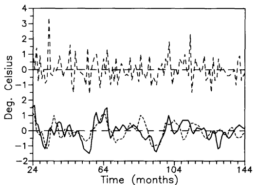
Fig. 3. An arbitrary portion of the time series (normalized by its standard deviation) of SSTA data (solid line) and of a realization of model III (dashed line), at the grid point at ( 175^\circ\text{W} , 30^\circ ). The computed time series of the forcing at this point is shown vertically displaced (long-dashes).
