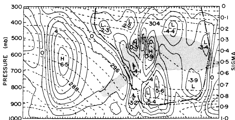
Fig. 9. As in Fig. 3c but for Exp. ICE (with ice microphysics).
