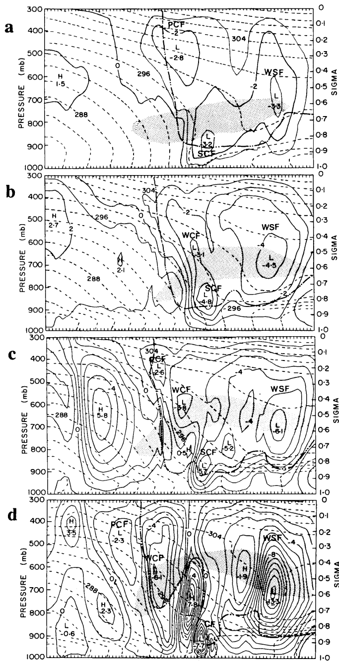
Fig. 3. Vertical cross section of vertical motion ( \omega , solid lines) at intervals of 1 \mu b s^{-1} and equivalent potential temperature (dashed lines) at intervals of 2 K along the central line of the FGM from (a) 12 h, (b) 16 h, (c) 18 h and (d) 21 h simulations of the Eady wave, corresponding to the Eady wave solution at t = 72, 76, 78 and 81 h, respectively. The dot-dashed line denotes cloud boundary and shadings indicate regions of negative MPV. The intervals marked on the low and upper frames are fine-mesh grids (i.e., 12 km), similarly in the rest of figures.
