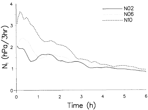
Fig. 7. Time evolution of the mean absolute surface pressure tendency N_1 (hPa/3 h). The parameters are the same as in the experiment IIR, except for the filter order: N02: 2nd order; N06: 6th order; N10: 10th order.
