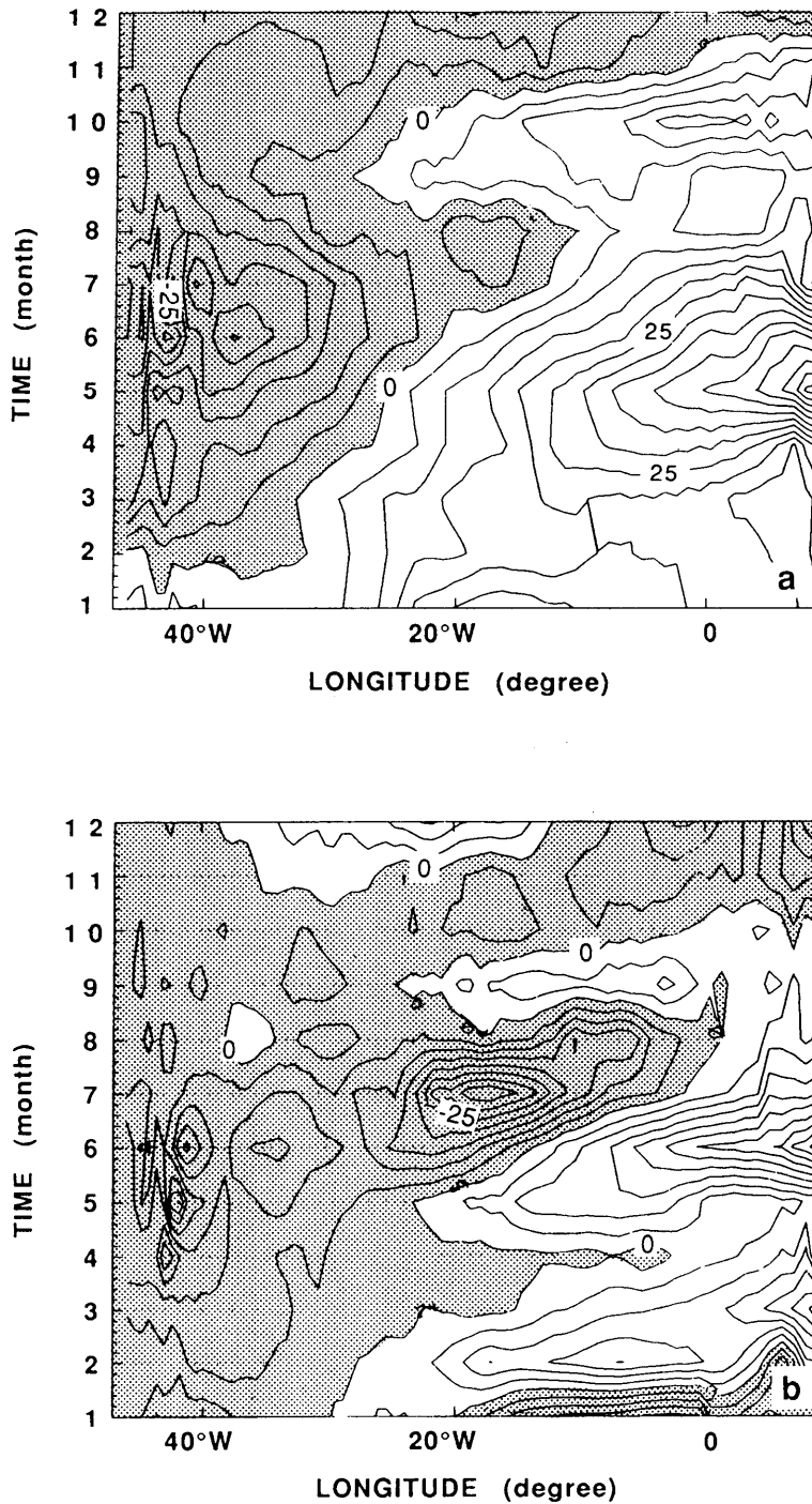
Fig. 11. Time-series along the equator of the difference of the depth of the 20°C between year 1984 and year 1983 for OWR (a) and OPR (b). Shaded area corresponds to a deeper level in 1983 than in 1984. The contour interval is 5 m.
