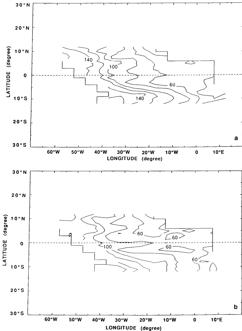
Fig. 7. Depth of the 20°C isotherm for April 1983 (a) and April 1984 (b) from observations. The contour interval is 20 m.
