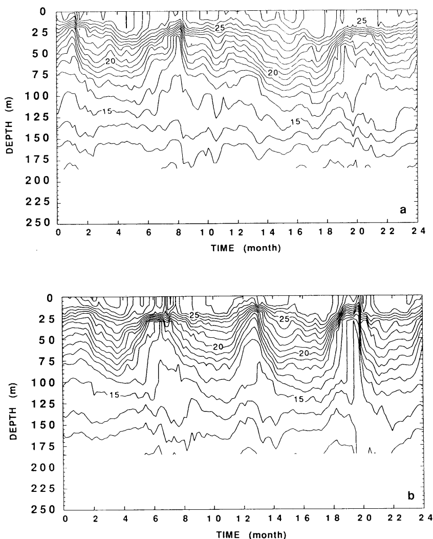
Fig. 10. Evolution in function of time (for 1983–1984) of the temperature profile at 0^\circ , 4^\circ\text{W} , for OWR simulation (a) and for OPR simulation (b). The contour interval is 1^\circ\text{C} .
