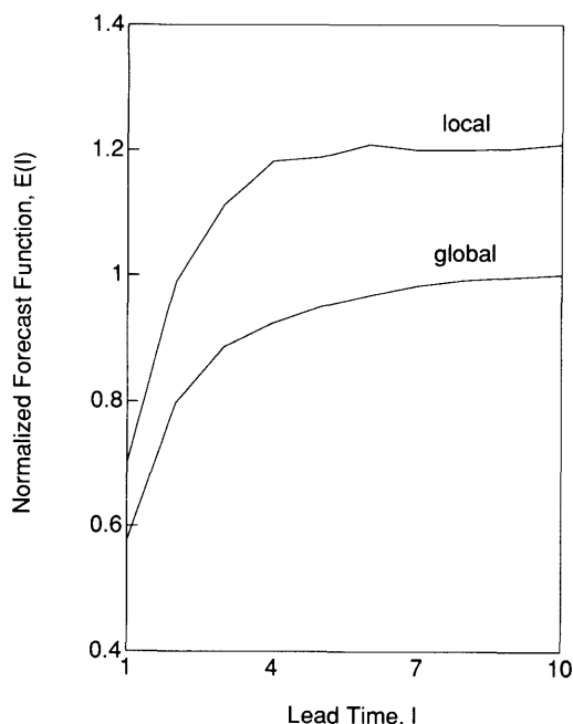
Fig. 8. Results of forecasting the residual time series.
