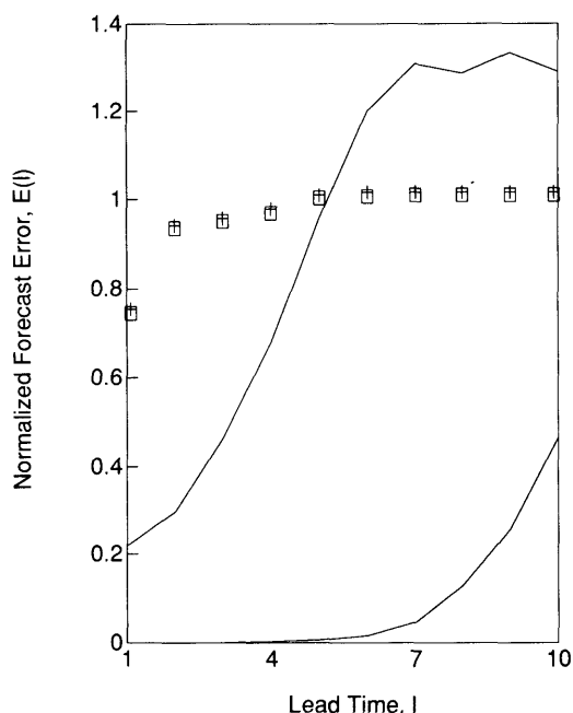
Fig. 1. Logistic map with a = 3.821 . Figure shows the normalized forecast error function against the lead time l . The lower solid curve refers to the local predictor and 0% external noise added; the other solid line refers to the local predictor but for an error level of 10%. The two curves corresponding to the global predictor are drawn with open squares (0% error) and plus signs (10% error).
