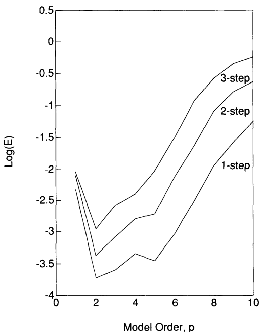
Fig. 2. Logistic map with a = 3.821 ; no external noise added. Figure shows the 1-step, 2-step and 3-step ahead normalized forecast error against the model order, p . The cases shown in figure refers to the local procedure.
