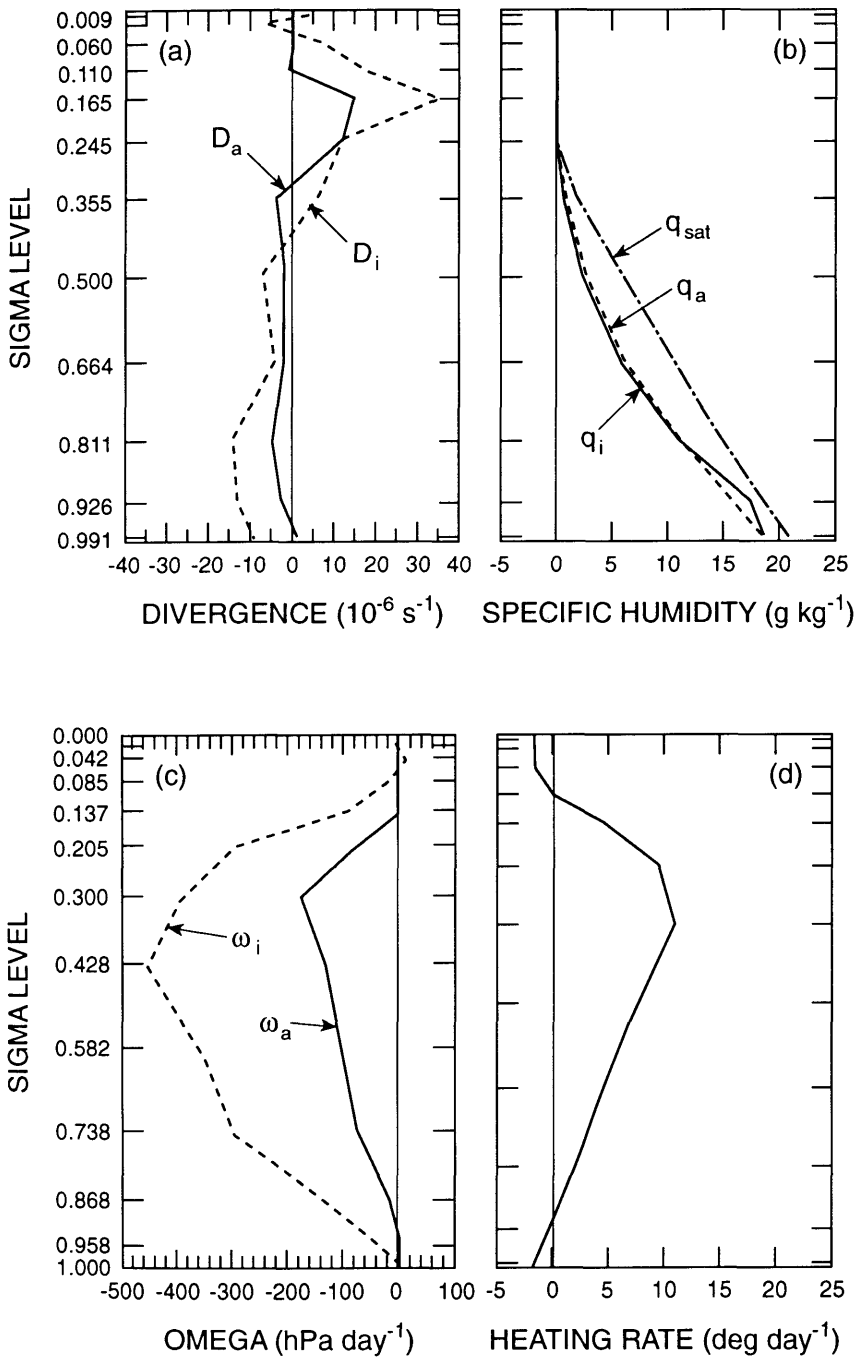
Fig. 9. Vertical distributions of various meteorological variables at longitude 154.7°E and latitude 9.8°S. (a) Input divergence D_i and adjusted value D_a , (b) input specific humidity q_i , adjusted value q_a , and saturated specific humidity q_{\text{sat}} , (c) input vertical p -velocity \omega_i and adjusted value \omega_a , and (d) diabatic heating rate.
