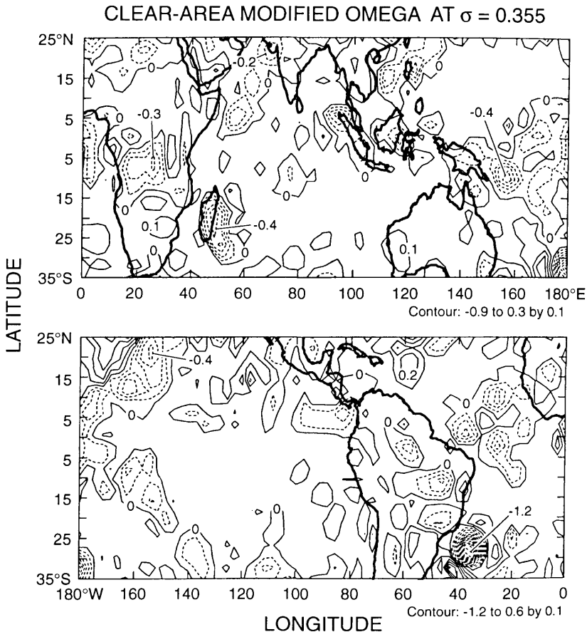
Fig. 5. Clear-area modified p -velocity at sigma level \sigma = 0.355 for 1200 UTC 1 January 1988. Contour interval is same as in Fig. 3.
