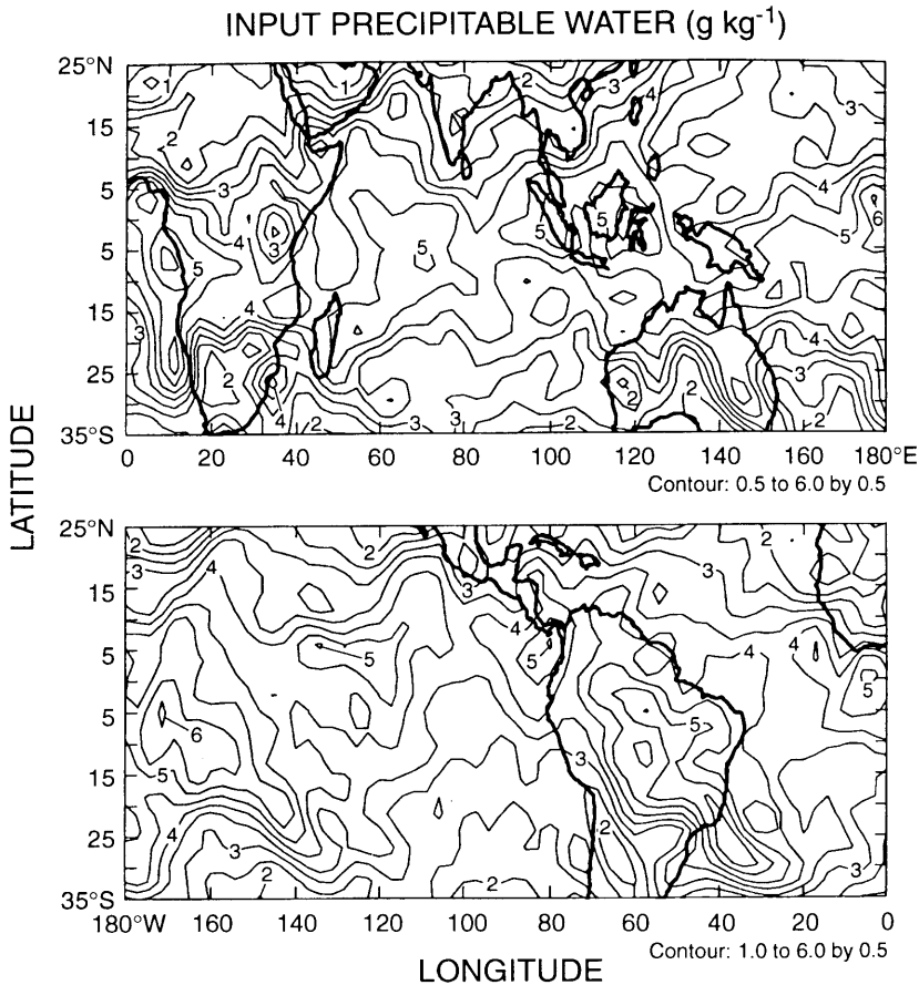
Fig. 6. Input precipitable water distribution for 1200 UTC 1 January 1988. Contour interval is 0.5 g kg -1 .
