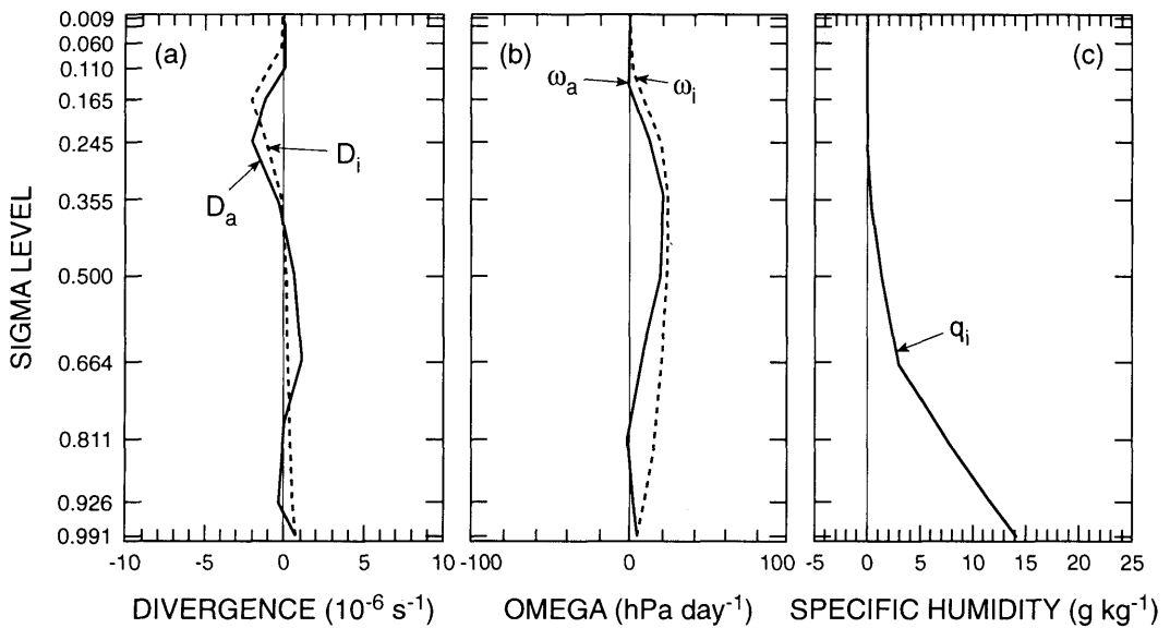
Fig. 12. Same as Fig. 10, except that averaging is taken over the downward-motion area.
