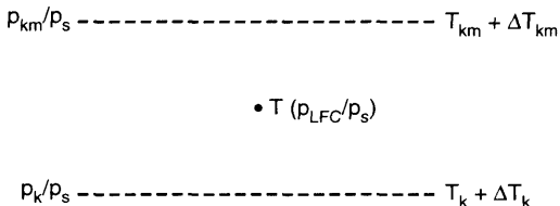
Fig. 1. Adjustment of environmental temperature at model levels p_{\text{km}}/p_{\text{s}} and p_{\text{k}}/p_{\text{s}} to ensure that T is less than T_{\text{c}} at p_{\text{LFC}}/p_{\text{s}} .
