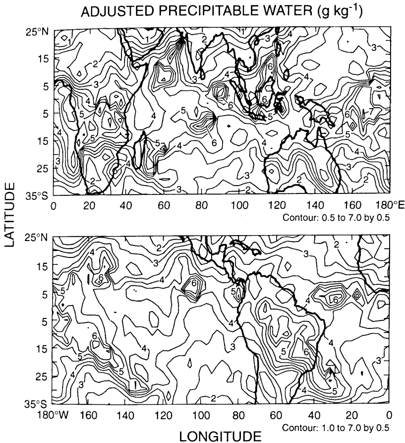
Fig. 7. Adjusted precipitable water distribution for 1200 UTC 1 January 1988. Contour interval is same as in Fig. 6.
