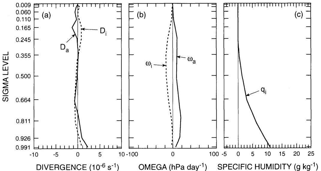
Fig. 13. Same as Fig. 10, except that averaging is taken over the convective fringe area.
