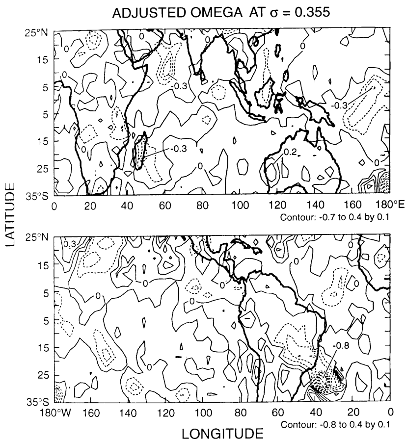
Fig. 4. Adjusted vertical p -velocity at sigma level \sigma = 0.355 for 1200 UTC 1 January 1988. Contour interval is same as in Fig. 3.
