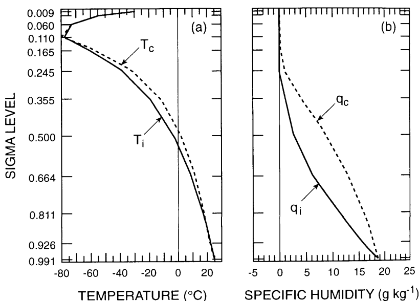
Fig. 8. (a) Vertical distributions of input large-scale temperature T_i and cloud temperature T_c at longitude 154.7°E and latitude 9.8°S. (b) Same as (a) except for input large-scale specific humidity q_i and cloud specific humidity q_c .
