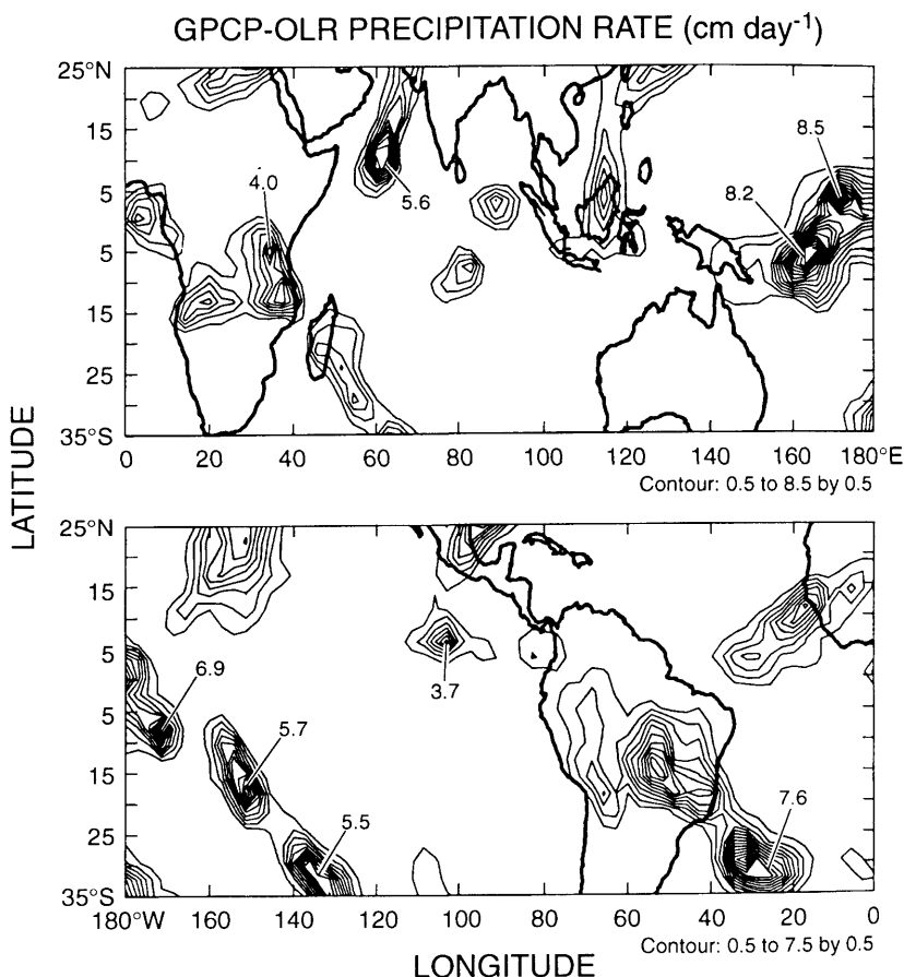
Fig. 2. Geographical distribution of precipitation rate in the tropics in \text{cm day}^{-1} for 1200 UTC 1 January 1988. Contour interval is 0.5 \text{ cm day}^{-1} .
