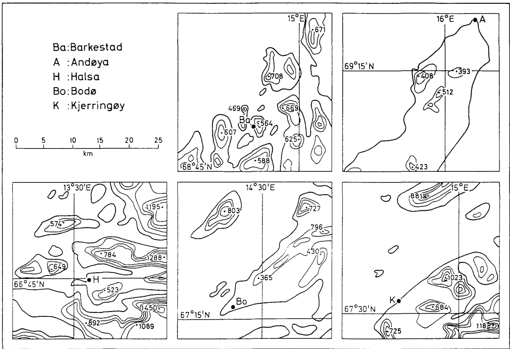
Fig. 5. Maps showing the topography of an area approximately 25 \times 25 km surrounding each of the 5 stations (200 m contours).
