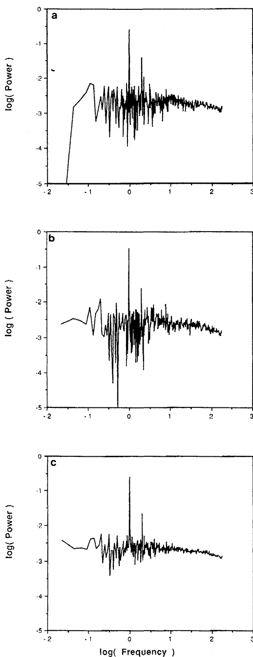
Fig. 2. Single station spectra of daily rainfall totals (Prague) of 4 consecutive 45-year subsets: (a) The first and (b) the last set; (c) the ensemble mean of all 4 subsets.
