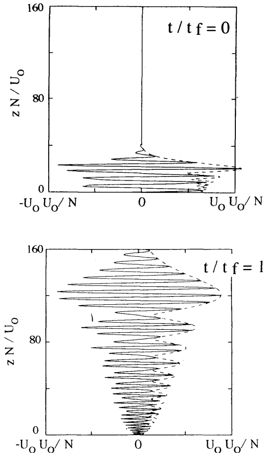
Fig. 2. Single harmonic mountain, \varepsilon = 43.2 ( t_f = 9 \text{ h} ), time evolution of the function \Psi_1 \exp(Z/2H) (solid line) and of its amplitude \langle \Psi_1 \rangle \exp(Z/2H) (dashed line).
