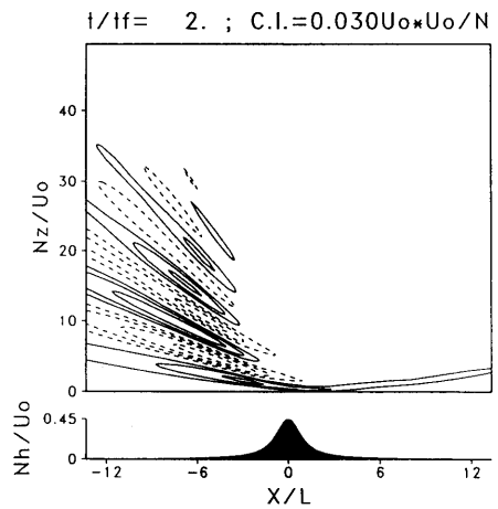
Fig. 10. Same as Fig. 7 for \epsilon = 4.8 ( t_f = 1 h).
