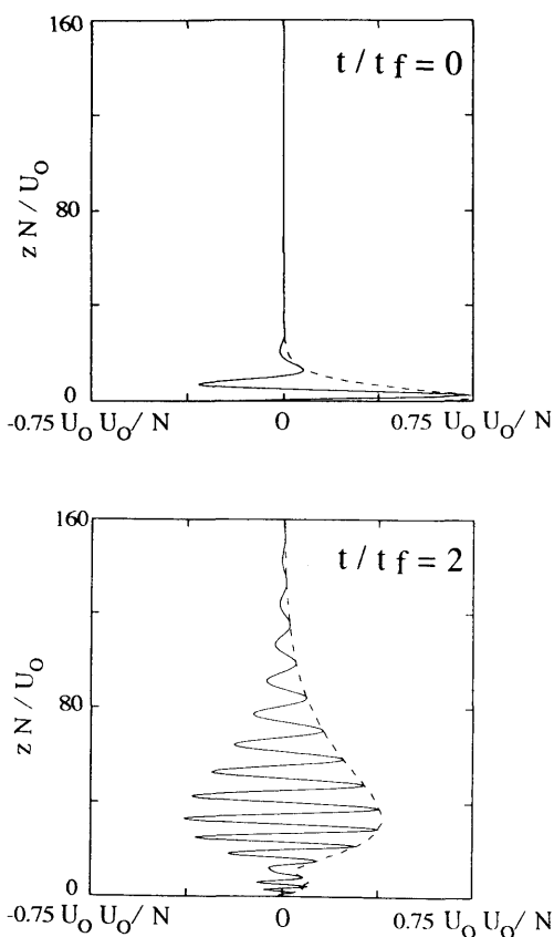
Fig. 4. Same as Fig. 2 for \varepsilon = 4.8 ( t_f = 1 h).
