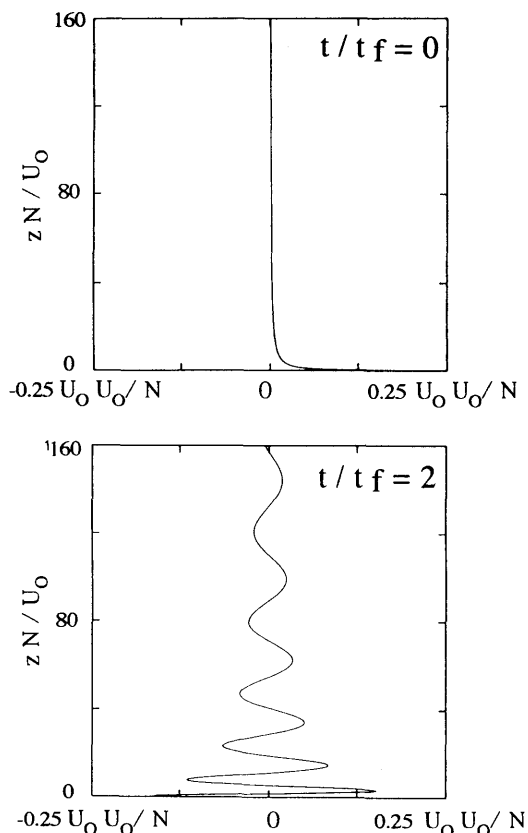
Fig. 14. Single harmonic mountain, ground generated disturbance in a fluid at rest, \varepsilon = 0.4 ( t_f = 5 min): time evolution of the function \Psi_1 . The Boussinesq and hydrostatic approximations are adopted.
