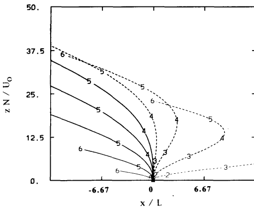
Fig. 6. Rays of wave packet propagation in the (x, z) plane, \varepsilon = 43.2 ( t_f = 9 h), k = 1/L . The dashed lines show the packets generated during the ascending phase of the wind; the dashed lines show the packets generated during the descending phase of the wind. The numbers characterize the location attained by each packets at the times: (2) t = -t_f/3 , (3) t = 0 , (4) t = t_f/3 , (5) t = 2t_f/3 , (6) t = t_f .
