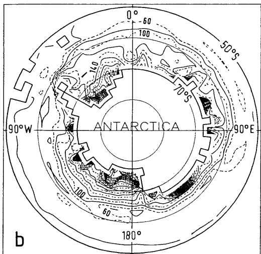
Fig. 4. Contours of oceanic mixed-layer depth (increment: 20 m) from the same model version and for the same dates as in Fig. 2.
