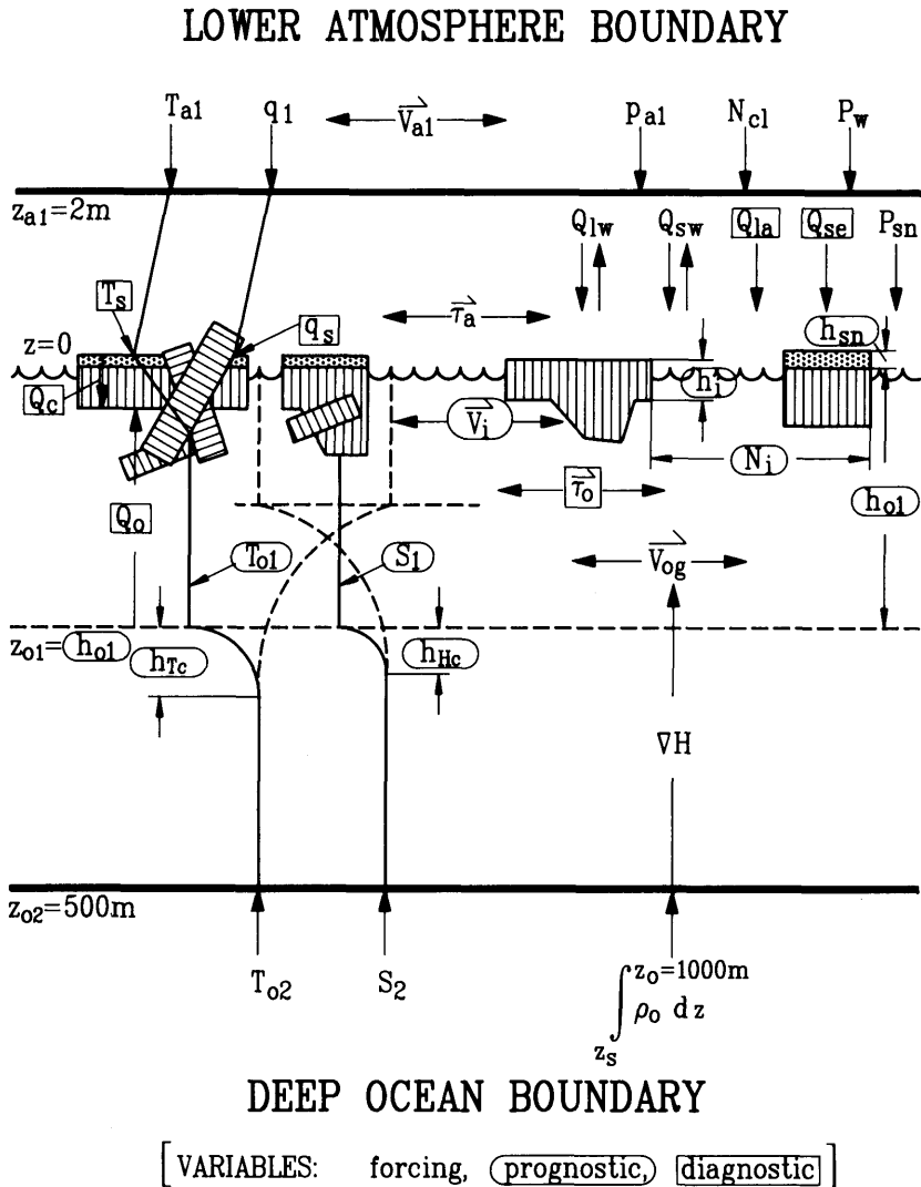
Fig. 1. Viewgraph of the variables of the SI-OML model.
