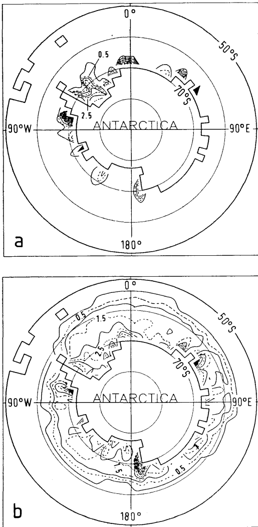
Fig. 7. Ice-thickness contours simulated with the ASL-SI-OML model, otherwise like Fig. 2.
