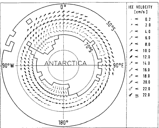
Fig. 8. Monthly mean ice velocities from the same model version as in Fig. 7, otherwise like Fig. 3b.
