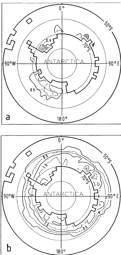
Fig. 13. Ice-thickness contours from the same model version as in Fig. 12, with employment of additional wind turning, otherwise like Fig. 2.
