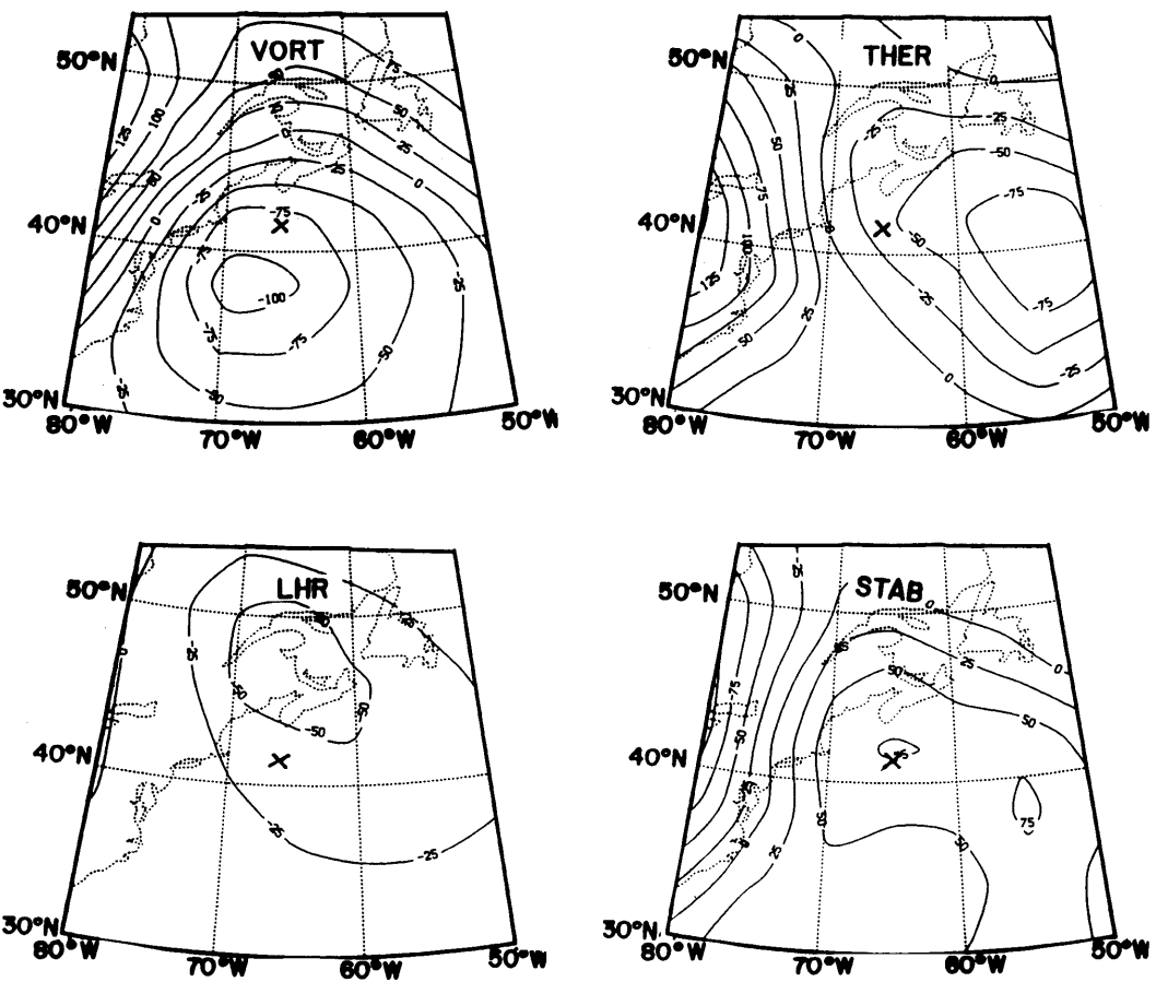
Fig. 5. Height tendencies ( \text{m } 12 \text{ h}^{-1} ) at 950 mb for 1200 GMT 18 January. X indicates the surface cyclone center. Upper left: Height tendency due to vorticity advection (VORT). Upper right: Height tendency due to temperature advection (THER). Lower left: Height tendency due to latent heat release (LHR). Lower right: Height tendency due to adiabatic temperature change (STAB).
