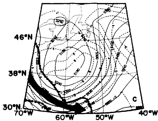
Fig. 2. 500 mb height (m, solid) and relative vorticity ( 10^{-5} \text{ s}^{-1} , dashed) and 300 mb jet axis (heavy arrow) and 50 \text{ ms}^{-1} isotach (heavy dashed) for the same map times as in Fig. 1.
