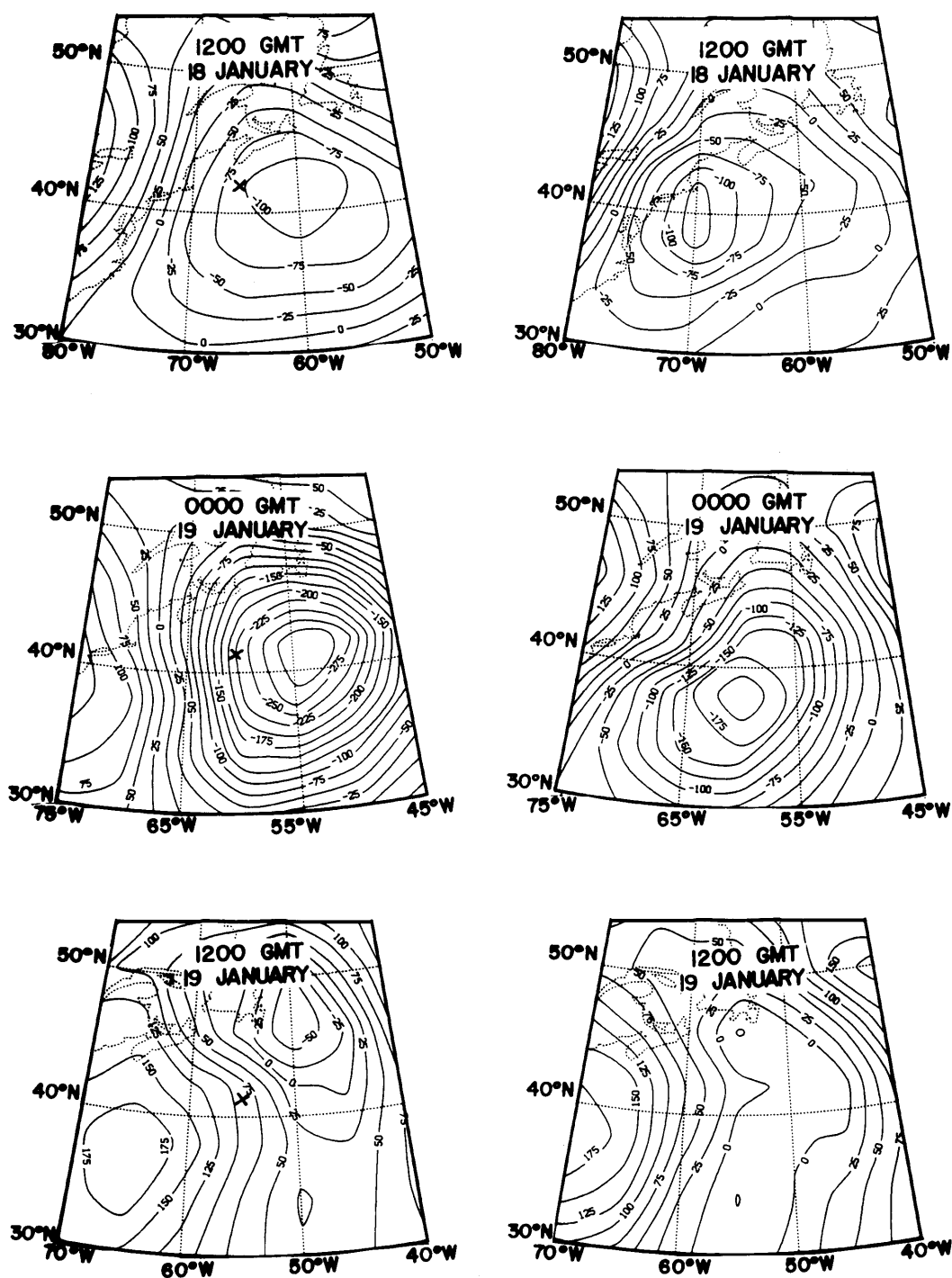
Fig. 4. Total calculated height tendencies (m 12 h -1 ) determined from (1) or (5). Left column 950 mb, right column 500 mb. X indicates the surface cyclone center.
