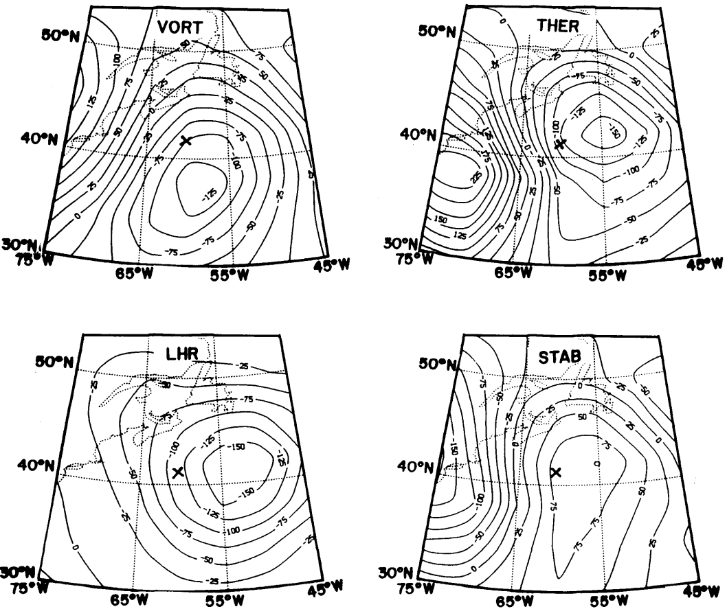
Fig. 7. As in Fig. 5 for 0000 GMT 19 January.
