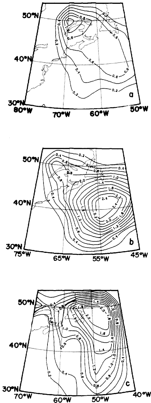
Fig. 3. Precipitation rates ( \text{mm h}^{-1} ) derived from the latent heat release computational scheme (see text) for the same map times as in Fig. 1.
