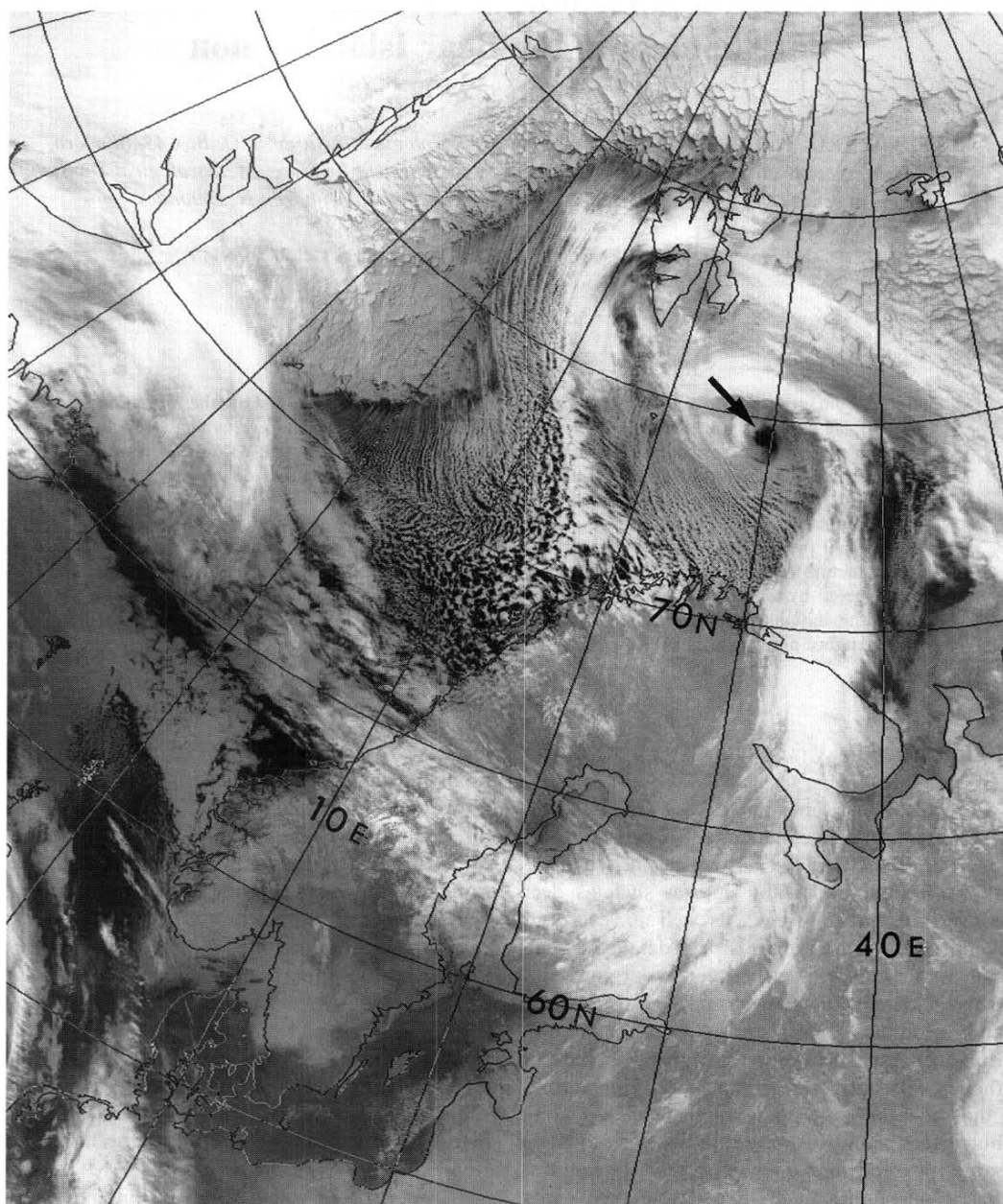
Fig. 1. NOAA-9 satellite image (infrared, Channel 4) 1244 UTC 26 February 1987 showing the incipient stage of the polar low which forms around the central dark eye (marked by arrow). Photograph courtesy of Department of Electrical Engineering and Electronics, University of Dundee.
