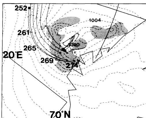
Fig. 13. Surface air trajectories ending up in the vicinity of the low at 0300 UTC 27 February 1987. The numbers along the trajectory are equivalent potential temperature after 0, 6, 9, 12 and 15 h of integration. Areas with heavy precipitation ( >1 mm/3 h) are stippled. Mean sea level pressure after 15 hours of integration valid at 0300 UTC 27 February 1987 is indicated by stippled lines at contour intervals of 2 hPa.
