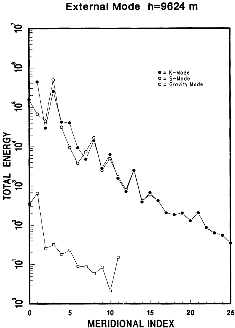
Fig. 4. Spectral distributions of atmospheric total energy of zonal wavenumber zero as functions of the meridional index l for the external mode ( k = 0 ). Units are Jm^{-2} . Dots denote for the K-modes, circles for S-modes, and squares for gravity modes.
