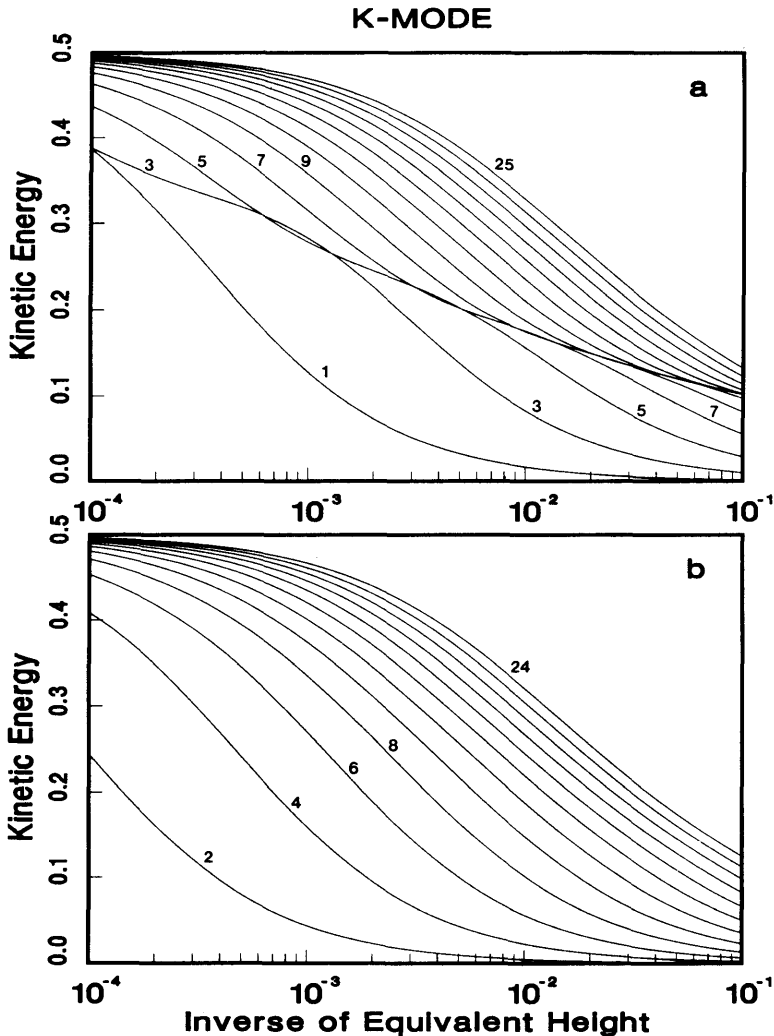
Fig. 1. Normalized kinetic energy of the K-modes as functions of equivalent height h_k . (a) Symmetric modes with odd meridional indices, l_R = 1, 3, 5, \dots , and (b) antisymmetric modes with even indices, l_R = 2, 4, 6, \dots .
