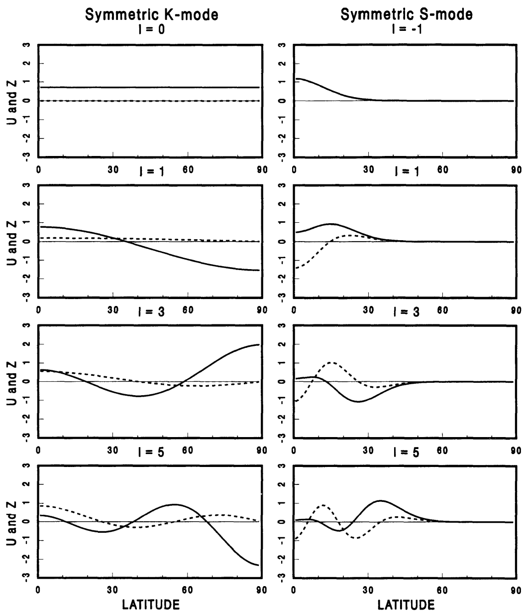
Fig. 6. Meridional structures of symmetric K-modes (left) and S-modes (right) for the internal component at h_k = 150 m. Solid lines denote the dimensionless geopotential Z , and dashed lines the dimensionless zonal wind U . Note that the first meridional index is l_R = 0 for the K-modes whereas l_R = -1 for the S-modes.
