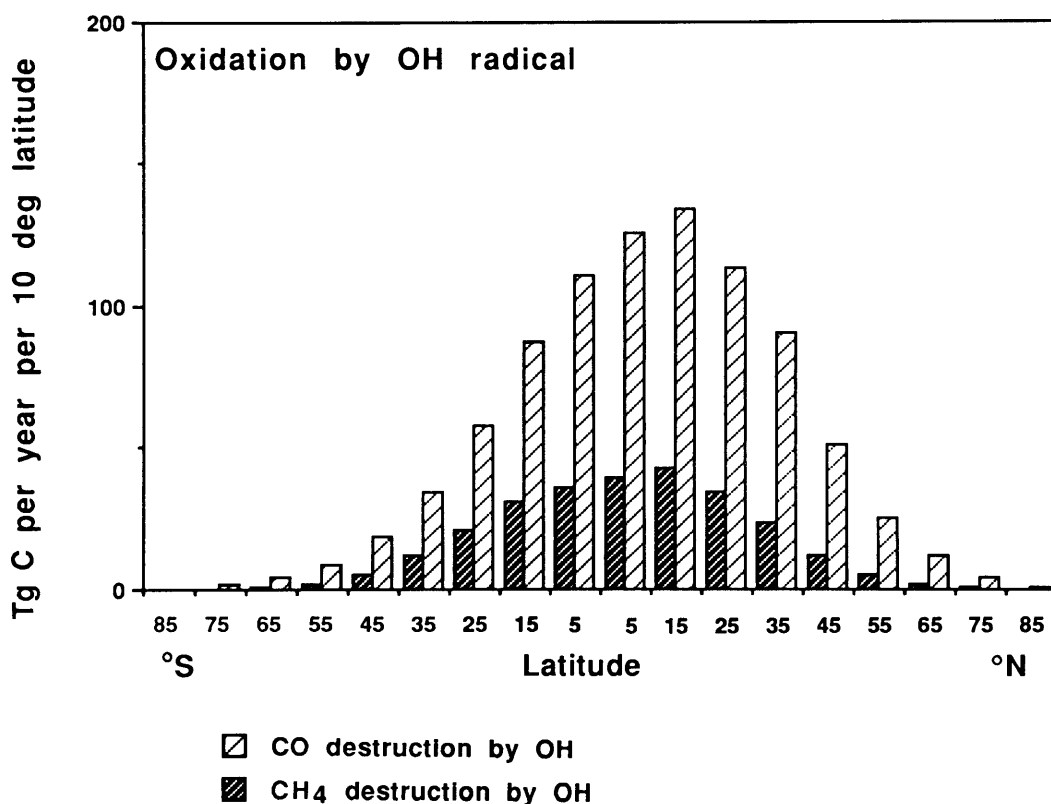
Fig. 7. Estimates of annual CO and \text{CH}_4 oxidation amounts by reaction with OH for 10^\circ latitude belts. The calculated total tropospheric destructions are 2050 Tg CO/yr and 360 Tg \text{CH}_4 /yr. Units: Tg C/yr.
