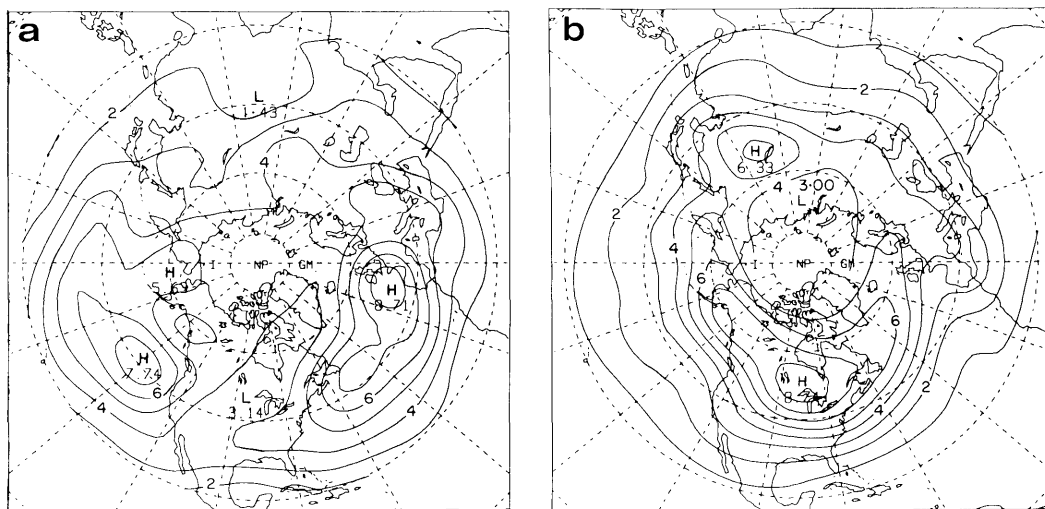
Fig. 3. Vertically integrated energetics of winter ECMWF low frequency disturbances. (a) KE , with a contour interval of 10^5 \text{ J/m}^2 ; (b) APE , with a contour interval of 10^5 \text{ J/m}^2 ; (c) AK , with a contour interval of 0.5 \text{ W/m}^2 ; (d) LK , with a contour interval of 1.0 \text{ W/m}^2 ; (e) BT , with a contour interval of 0.5 \text{ W/m}^2 and (f) NK , with a contour interval of 1.0 \text{ W/m}^2 .
