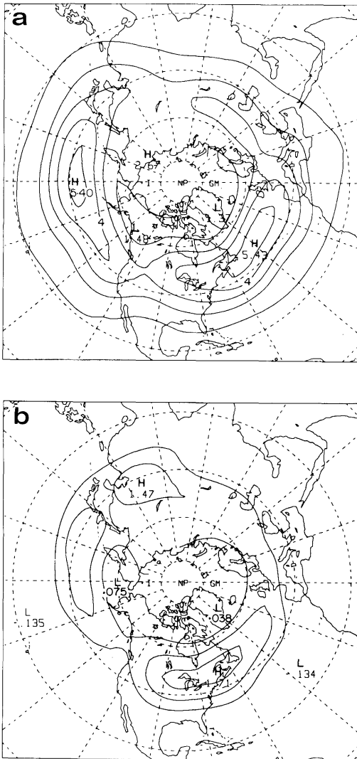
Fig. 4. Vertically integrated energetics of summer ECMWF high frequency disturbances. (a) KE , with a contour interval of 10^5 \text{ J/m}^2 and (b) AK , with a contour interval of 0.5 \text{ W/m}^2 .
