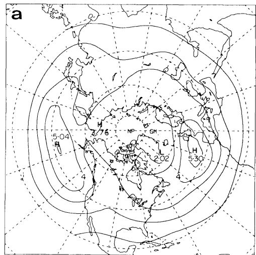
Fig. 5. Vertically integrated energetics of summer ECMWF low-frequency disturbances. (a) KE , with a contour interval of 10^5 \text{ J/m}^2 , (b) APE , with a contour interval of 10^5 \text{ J/m}^2 , (c) AK , with a contour interval of 0.5 \text{ W/m}^2 , (d) LK , with a contour interval of 0.5 \text{ W/m}^2 and (e) LK + NK , with a contour interval of 0.5 \text{ W/m}^2 .
