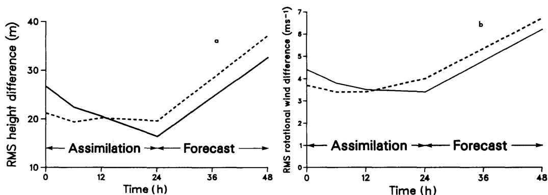
Fig. 9. (a) Temporal variation, over the assimilation period (from 0 to 24 h) and over a subsequent 24-h forecast (from 24 to 48 h), of the root-mean-square difference between (i) the height fields of a model solution produced by variational assimilation and (ii) the corresponding 500 mb height fields of the operational EMERAUDE analyses. Dashed curves: assimilation with constant temporal weighting of the observations. Full curves: assimilation with variable weighting of the observations. (b) As (a) but for rotational wind root-mean-square difference.
