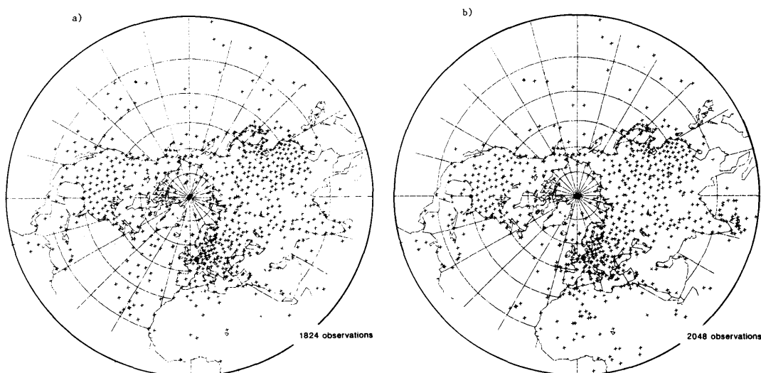
Fig. 1. Geographical distribution of the height and wind observations used in the assimilation experiments (panels (a) and (b) respectively). Most of the height observations over the Atlantic Ocean have been obtained from SATEM thicknesses.
