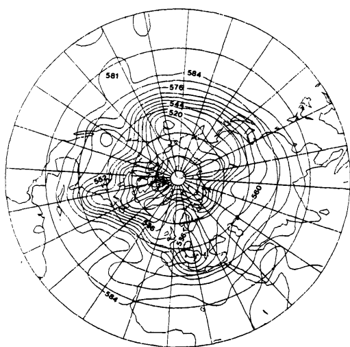
Fig. 3. 500 mb height field for 00:00 GMT, 19 March 1985, as produced by the operational assimilation and forecast EMERAUDE system of Direction de la Météorologie, Paris (unit: dam).
