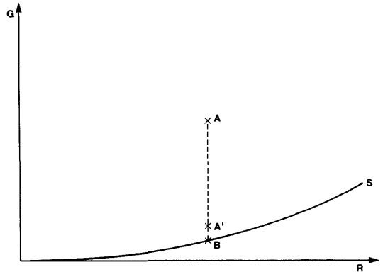
Fig. 6. Schematic representation of the phase space E , extracted from Leith (1980). Each point in E is defined by its projections R and G onto the subspaces spanned by the Rossby modes and gravity modes respectively. S is the slow manifold, i.e., the subset of points satisfying condition (5.2). Starting from a given point A , the Machenhauer nonlinear normal mode initialization algorithm would lead, in the limit of infinitely many iterations, to point B , located on the slow manifold. Because the algorithm must in practice be interrupted after a finite number of iterations, it only leads to point A' .
