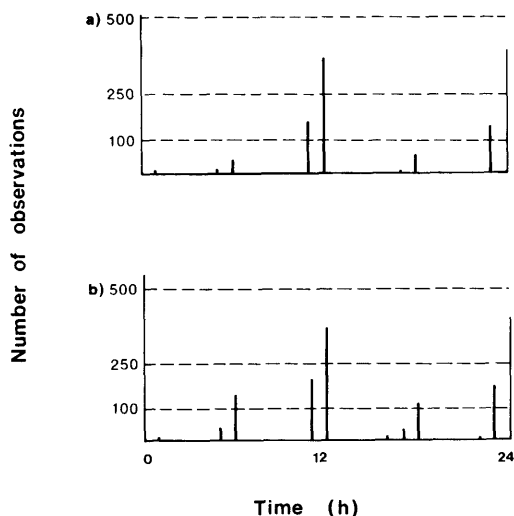
Fig. 2. Temporal distribution of the observations used in the assimilation experiments (observation time rounded up to the nearest full hour). Vertical coordinate is number of observations: (a) height observations; (b) wind observations.
