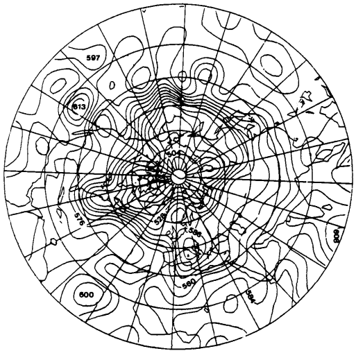
Fig. 4. Height field produced at the end of the assimilation period (00:00 GMT, 19 March 1985) by minimization of the distance function (5.1) (unit: dam).
