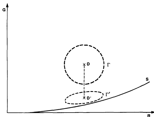
Fig. 7. Same schematic representation of the phase-space E as in Fig. 6. Points D and D' correspond respectively to the “uninitialized” and “initialized” model states leading to the solution which minimizes the distance function penalized by term (5.3). D' is the image of D through the Machenhauer algorithm. Similarly, \Gamma and \Gamma' are level curves for the penalized distance function in the spaces of “uninitialized” and “initialized” model states respectively. \Gamma' is the image of \Gamma through the Machenhauer algorithm.
