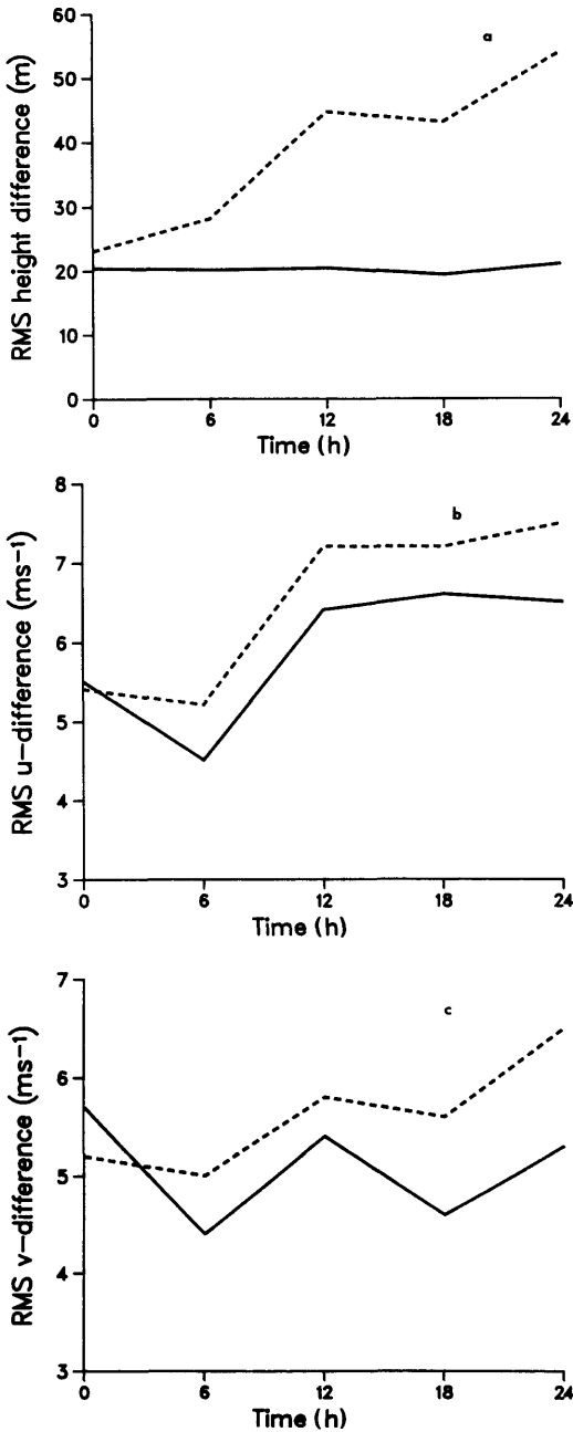
Fig. 5. Temporal variations, over the assimilation period (t_0, t_1) , of the root-mean-square differences between the observations and (i) the model solution produced from the EMERAUDE analysis at time t_0 (dashed curves) (ii) the model solution minimizing the distance function (5.1) (full curves). Panel (a): height (m). Panel (b): eastward ( u ) component of the wind ( \text{m s}^{-1} ). Panel (c): northward ( v ) component of the wind ( \text{m s}^{-1} ).
