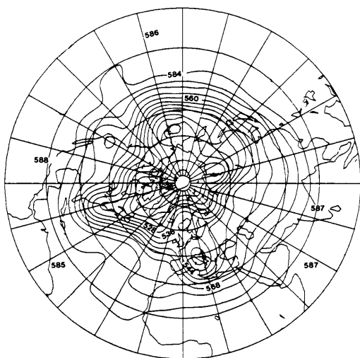
Fig. 8. As Fig. 4, but for a distance function penalized with term (5.3).
