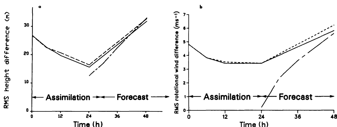
Fig. 10. As Fig. 9, but for assimilations without SATEM observations (dashed curves, identical with full curves of Fig. 9) and with SATEM observations (full curves). The dash-dotted curves show the time variation of the root-mean-square difference between (uninitialized) EMERAUDE analyses and a shallow-water forecast produced from the (initialized) EMERAUDE analysis at the end of the assimilation period. Panels a and b: height and rotational wind root-mean-square differences respectively.
