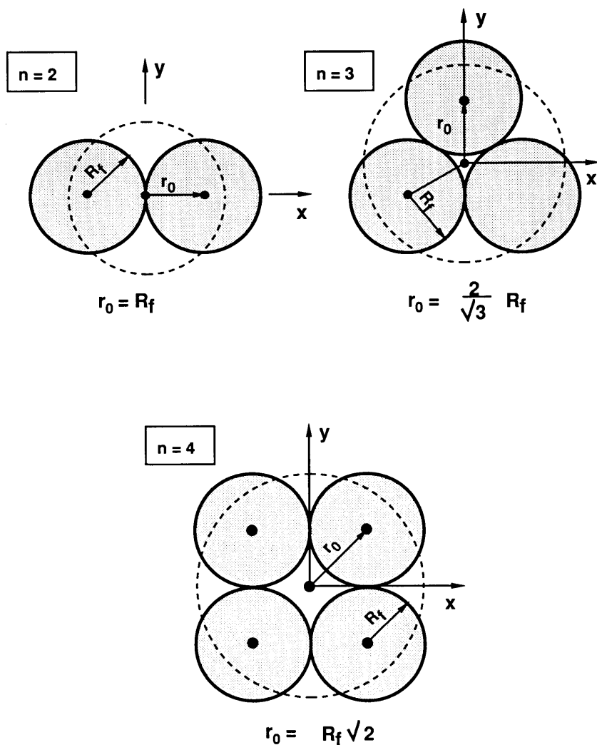
Fig. 4. The assumed final structure of the off-spring (i.e., the eddies resulting from the splitting). Three possible states are shown, n is the number of off-spring, r_0 is the distance from their center to the original center of rotation, and R_f is their radius. The dashed line shows the edge of the parent eddy.
