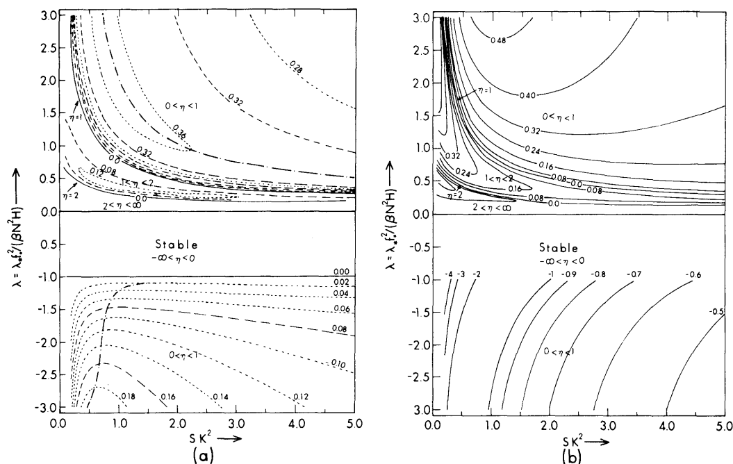
Fig. 1. Contour plot of (a) growth rate S^{1/2}kc , and (b) phase speed c_r , for an inviscid non-Boussinesq fluid as a function of non-dimensional vertical shear \lambda and total wave-number squared SK^2 . The dashed-dotted lines indicate the most unstable Charney mode.
