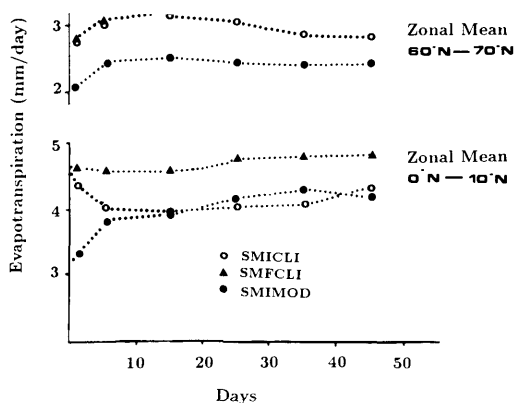
Fig. 3. Time evolution of the evaporation rate computed over land. Values are zonal means throughout the three experiments for two latitudinal bands: 0^{\circ}\text{N} – 10^{\circ}\text{N} and 60^{\circ}\text{N} – 70^{\circ}\text{N} . Experimental points are averages for days 0–2, 3–10, 11–20, 21–30, 31–40 and 41–50.
