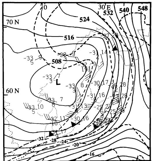
Fig. 1. The 500 mb geopotential height for 00 GMT, 23 October 1986 (solid lines: geopotential height in dam, dashed lines: temperature in °C).
