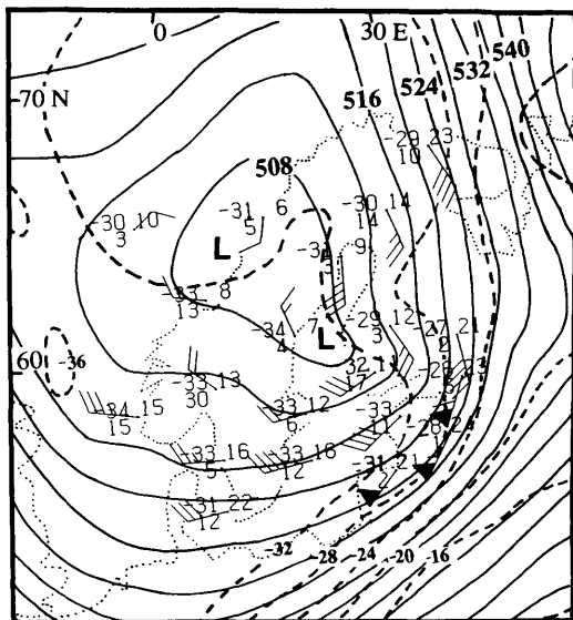
Fig. 8. The 500 mb analysis for 12 GMT, 23 October 1986. Notation as in Fig. 1.
