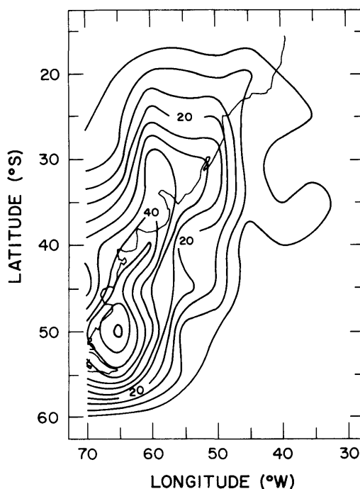
Fig. 3. Frequency of cyclogenesis. The contours represent the number of cyclones in a 5° longitude \times 5° latitude box during the 7-year period 1980–86. The contour interval is 5.
