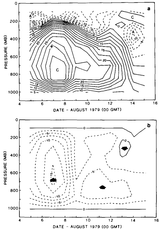
Fig. 2. Height-time section for Depression 1 (6–13 August 1979). (a) Relative vorticity ( 10^{-6} \text{ s}^{-1} ), and (b) vertical velocity ( 10^{-4} \text{ mb s}^{-1} ).
