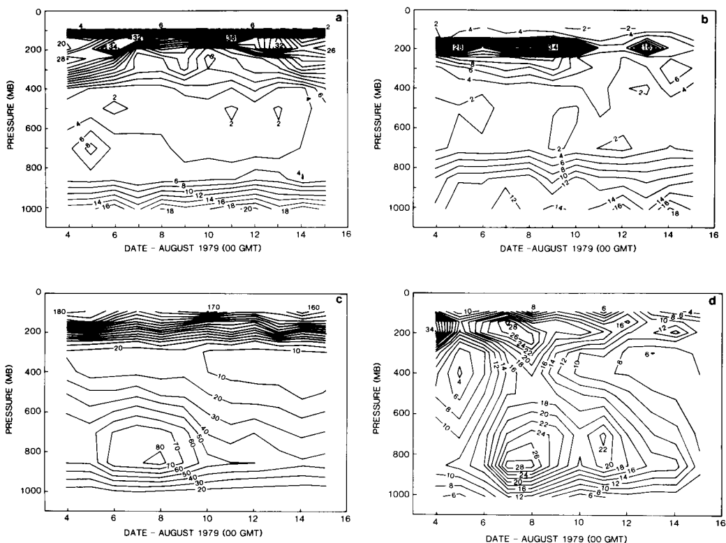
Fig. 6. Height-time section of (a) the zonal available potential energy; (b) eddy available potential energy; (c) zonal kinetic energy; (d) eddy kinetic energy. The units are \text{m}^2 \text{s}^{-2} .
