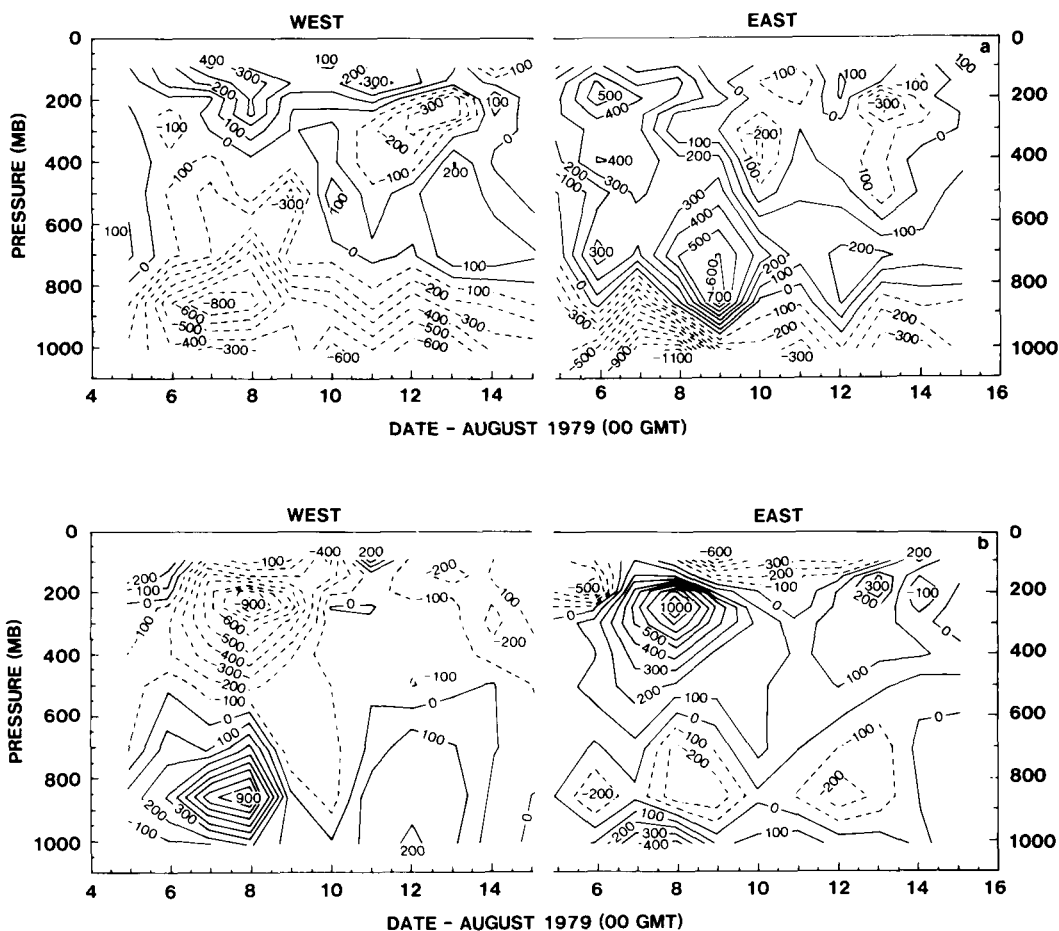
Fig. 4. Height-time section for Depression 1. The eastern and western sectors: (a) the vorticity divergence term; (b) horizontal advection term; (c) the vertical advection term; (d) the tilting term; (e) the residual term. The units are 10^{-12} \text{ s}^{-2} .
