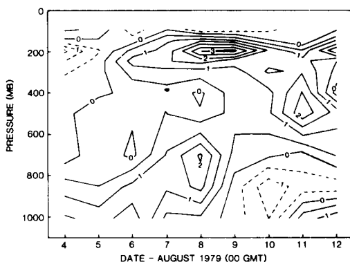
Fig. 10. Temperature anomaly ( ^{\circ}\text{C} ) for depression (4-12 August 1979).
