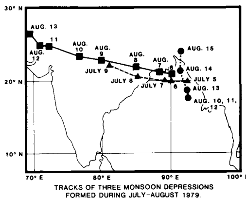
Fig. 1. Tracks of the three monsoon depressions formed during July–August 1979, and the area of study.
