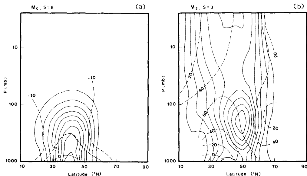
Fig. 5. Latitude-height structures of geopotential amplitudes (solid line in arbitrary unit) and phases (dashed line denoting longitudes of ridges) for (a) M_C at wavenumber s = 8 and (b) M_2 at s = 3 , with a basic state of Simmons and Hoskins' 30^\circ jet profile.
