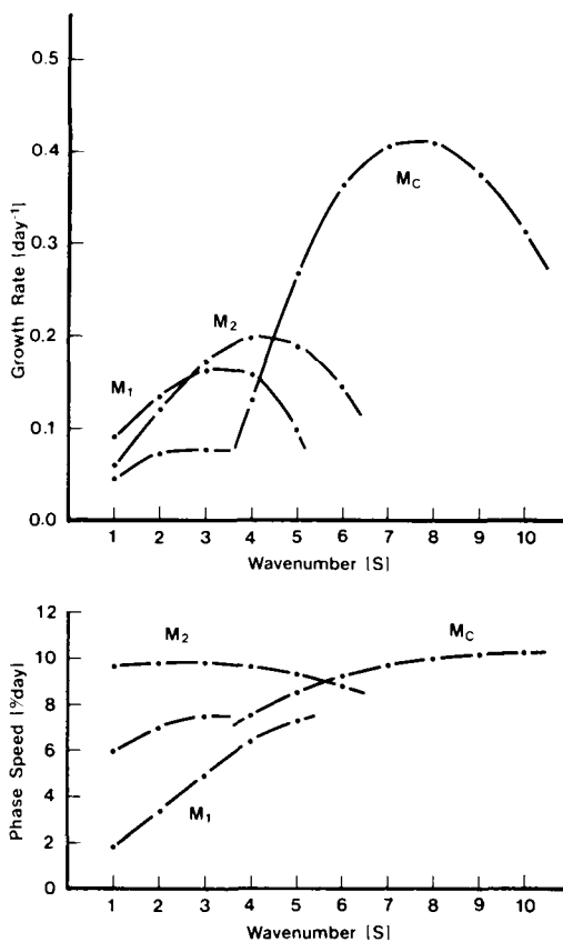
Fig. 4. As in Fig. 3 but for a zonal basic state of January 1979. M_C is the shallow Charney mode, and M_1 , M_2 the deep Charney modes.
