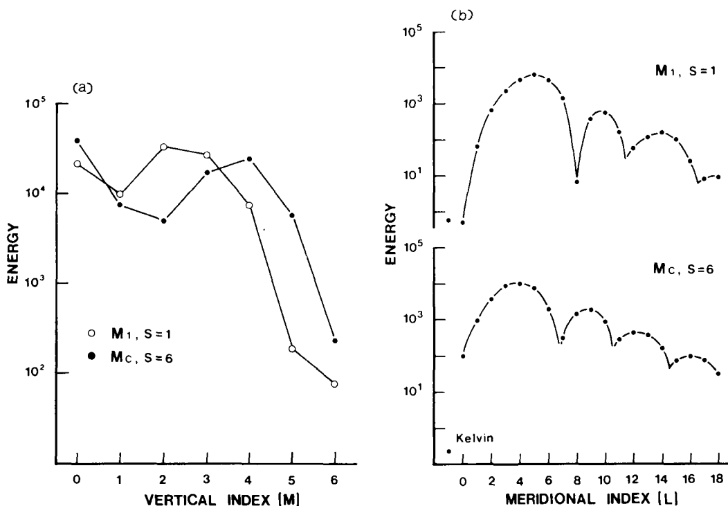
Fig. 7. Normalized energy spectra for M_1 at s=1 and M_C at s=6 (a) in the vertical index domain, resulting from the summation of all meridional indices, and (b) in the meridional index domain for the barotropic component.
