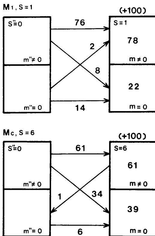
Fig. 8. Energy flow box diagrams for M_1 at s=1 and M_C at s=6 . Upper boxes ( m'' \neq 0, m \neq 0 ) denote the baroclinic components and lower boxes ( m''=0, m=0 ) the barotropic components. Left boxes ( s''=0 ) are zonal-mean components and the right boxes ( s=1 and 6 ) the eddy components. Energy transformations are normalized to yield the percentile contributions of the growth. Percentile energy is read in the boxes.
