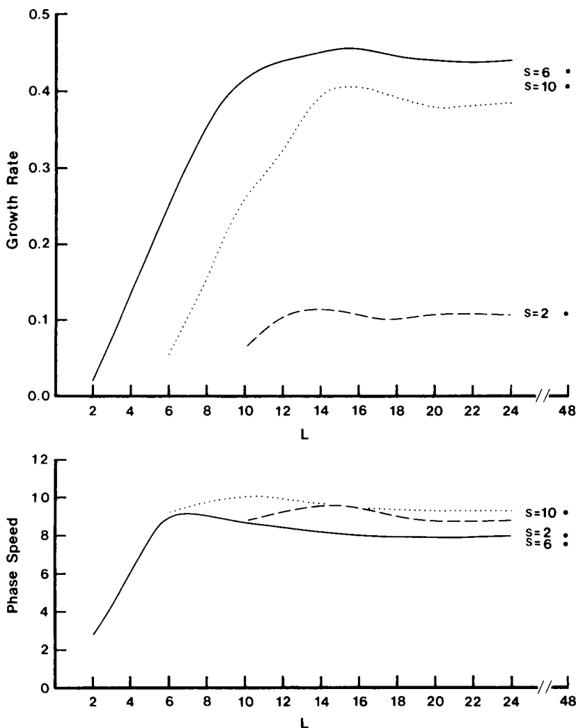
Fig. A2. Growth rates (day -1 ) and phase speeds (°/day) of the most unstable modes at wavenumbers s = 2, 6 , and 10 as functions of meridional truncations L . The dots at L = 48 represent the results including 24 gravity mode basis added with the Rossby mode basis of l = 0-24 .
