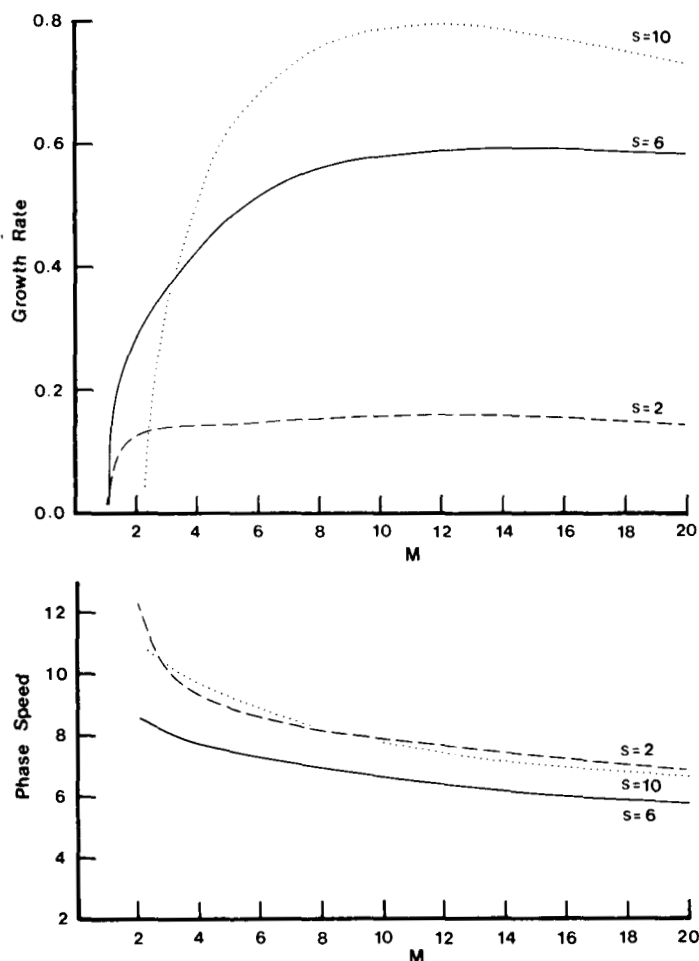
Fig. A1. Growth rates (day -1 ) and phase speeds C_R (m/s) of the most unstable modes at wavenumbers s = 2, 6 , and 10 as functions of vertical resolutions M .
