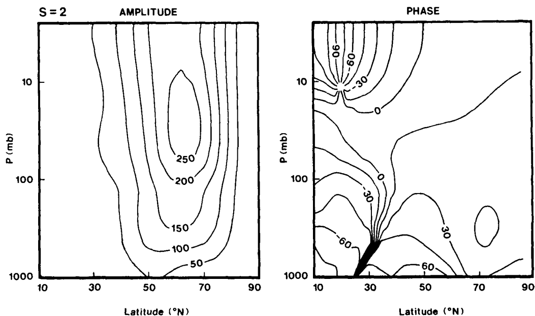
Fig. 9. Latitude-height section of geopotential height of the wavenumber 2 for January 1979 used as the basic state. Amplitude ( m ) and phase (longitude of ridge) are reproduced by the composition of m'' = 0-6 and l'' = 0-18 .
