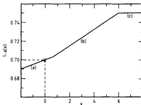
Fig. 3. Dependence of the coalbedo 1 - a(x) on the deviation of temperature from a reference value T_0 , represented by a cross on branch (a). The slope of 1 - a(x) changes at branch (b) and becomes temperature independent at higher x (branch (c)).
