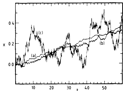
Fig. 1. Time evolution of the variable x obtained by numerical integration of eq. (2) with g = 1 and F(t) a Gaussian white noise: curve (a) q^2/C^2 = 6.9 \times 10^{-5} ; curve (b) q^2/C^2 = 2.8 \times 10^{-4} and curve (c) q^2/C^2 = 6.9 \times 10^{-3} \text{ year}^{-1} .
