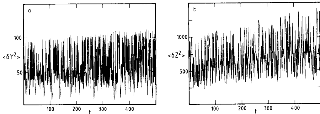
Fig. 10. Time evolution of the variance of the variables Y (a) and Z (b) around the averages of Fig. 9.
