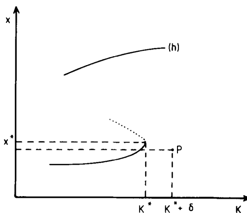
Fig. 6. Schematic representation of a limit-point bifurcation. Beyond the threshold value K^* of the control parameter, the system is bound to evolve to a new branch (h).
