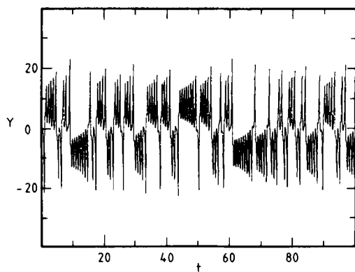
Fig. 8. Time evolution of the variable Y obtained by numerical integration of eqs. (22). Parameters used: \sigma = 10 , b = \frac{8}{3} and r = 26 .
