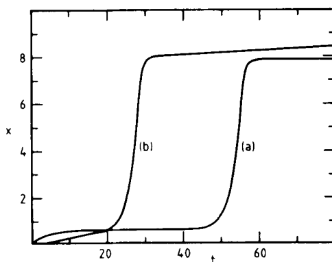
Fig. 5. Numerical integration of eqs. (15) with initial condition x = 0 . Curve (a): sudden increase of the CO 2 content above the critical point K = K^* + \delta with \delta = 10^{-4} . Curve (b): gradual increase, K = \tilde{K}et with \varepsilon = 0.01 \text{ year}^{-1} and \tilde{K}/C = 1 \text{ year}^{-1} .
