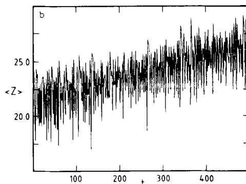
Fig. 9. The evolution of averages of the variables Y (a) and Z (b) over twice the pseudo-period of the system. Parameters as in Fig. 8 but r = 26 + \epsilon t with \epsilon = 0.01 .
