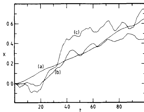
Fig. 2. As in Fig. 1, but with F(t) an Ornstein-Uhlenbeck noise and \gamma = 0.1 \text{ year}^{-1} ; curve (a) q^2/C^2 = 2.8 \times 10^{-6} ; curve (b) q^2/C^2 = 6.9 \times 10^{-5} and curve (c) q^2/C^2 = 2.8 \times 10^{-4} \text{ year}^{-3} .
