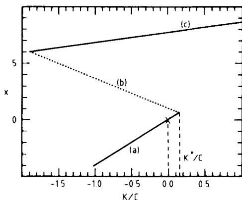
Fig. 4. Dependence of the steady state solutions of eqs. (15) on the CO 2 content K . The lower and intermediate branches merge at the critical value K^* . For the values of the parameters used, (a) and (c) are stable whereas (b) is unstable. The cross in branch (a) represents a reference state corresponding to pre-industrial climatic conditions.
