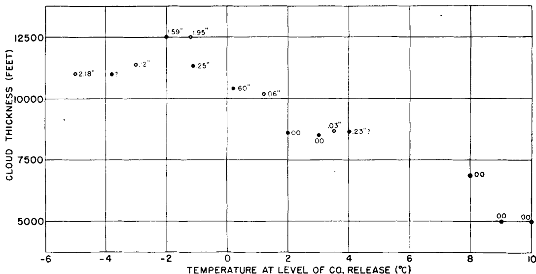
Fig. 1. Rainfall amounts associated with seeded clouds of given temperature and thickness. Temperature given are at the level of CO 2 release, approximately at the top of the cloud.
