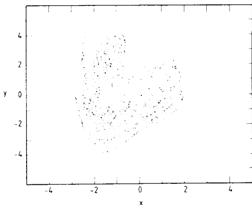
Fig. 7. Non-periodic attractor of system (8) for the parameter values of Fig. 4 except q = 20q_c .
