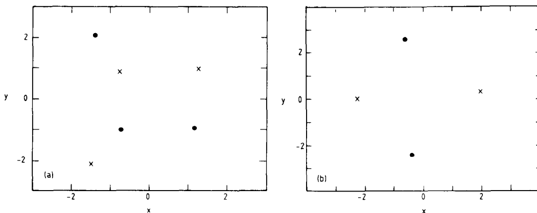
Fig. 5. Poincaré maps of the forced system eqs. (8) for the same parameter values as in Fig. 4 but with q = 12q_c . Depending on the initial conditions, the system evolves to one of the 4 coexisting attractors: (a) 2 different period-3 attractors; (b) 2 different period-2 attractors.
