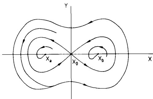
Fig. 1. Phase-space portrait of a 2-variable system involving a pair of homoclinic orbits.
