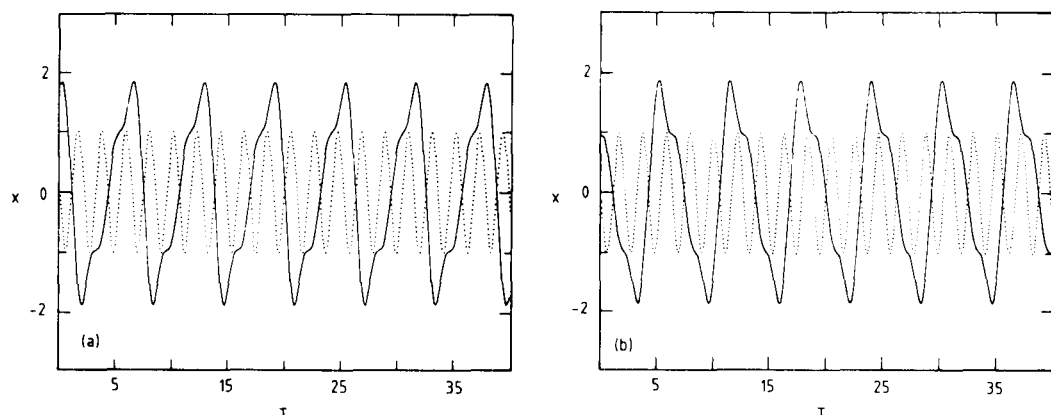
Fig. 6. Time dependence of variable x of the 2 period-3 solutions ((a) and (b)) for the same parameter values as in Fig. 4 but with q = 13.5q_c . The dotted line represents the forcing with amplitude normalized to unity. Notice that the 2 solutions exhibit different phase-shifts relative to the forcing.
