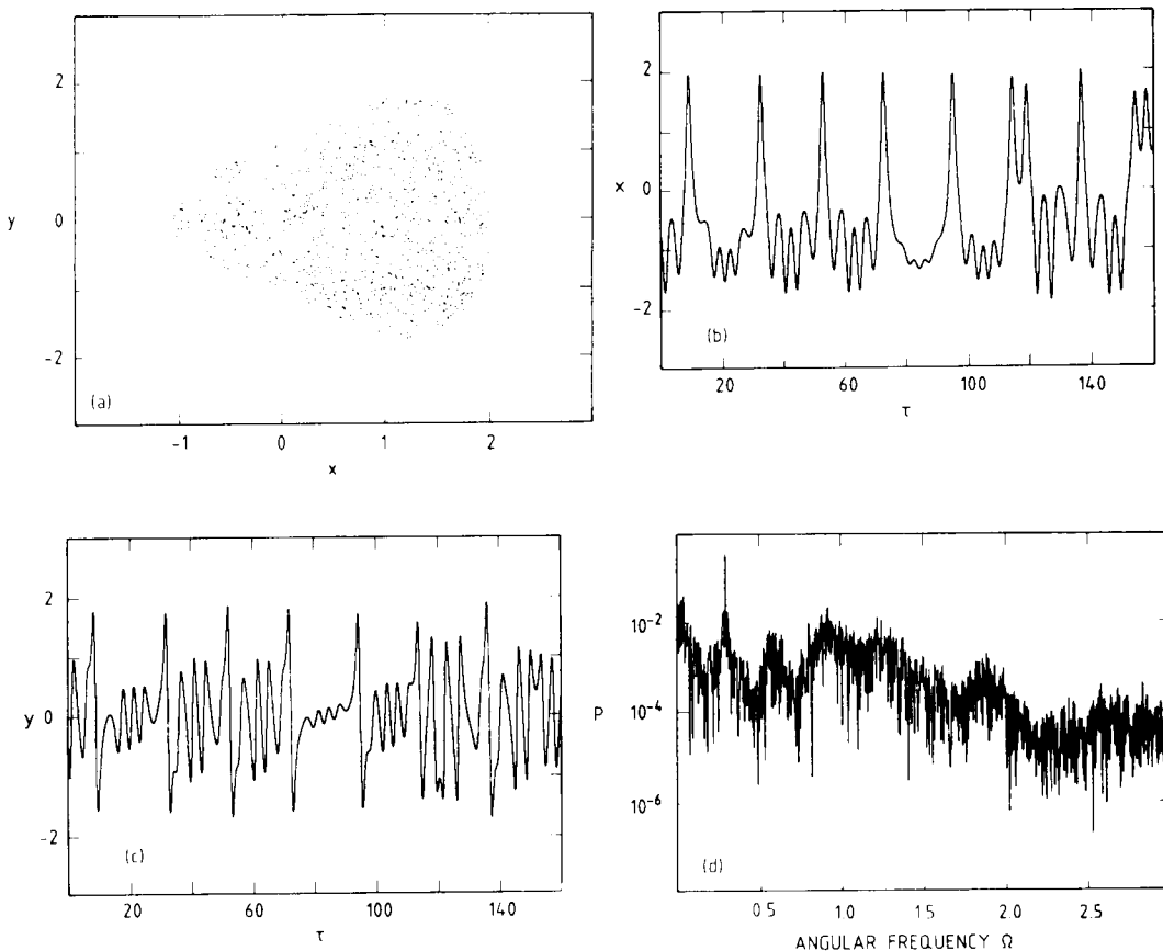
Fig. 8. Numerical integration of eqs. (8) for the same parameter values as in Fig. 4 but \Omega = 0.3 and q = 50q_c , where now q_c = 0.148 . (a) Poincaré map; (b) time evolution of variable x ; (c) time evolution of variable y ; (d) power spectrum of variable x .
