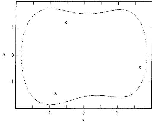
Fig. 4. Poincaré map of the forced system eqs. (8) for \gamma_2 = 1, \gamma_1 = 1.01, \mu = 0.1, \Omega = 3 and q = q_c + 0.2 , where q_c = 1.96 . Depending on the initial conditions, the system evolves either to a quasi-periodic attractor (closed curve) or to a periodic one, with a period 3 times as large as the forcing period (points and crosses).
