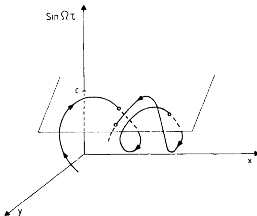
Fig. 3. Schematic representation of a Poincaré map for a forced system. As the system evolves, a representative trajectory cuts a plane of section C at discrete times \tau_n . The study of the dynamics on the surface of the section gives valuable information on the qualitative behavior of the initial system.
