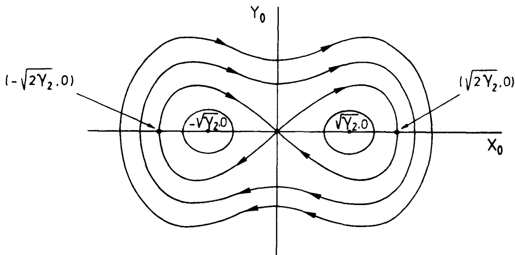
Fig. 2. Phase-space portrait of Duffing's oscillator for \gamma_2 > 0 .
