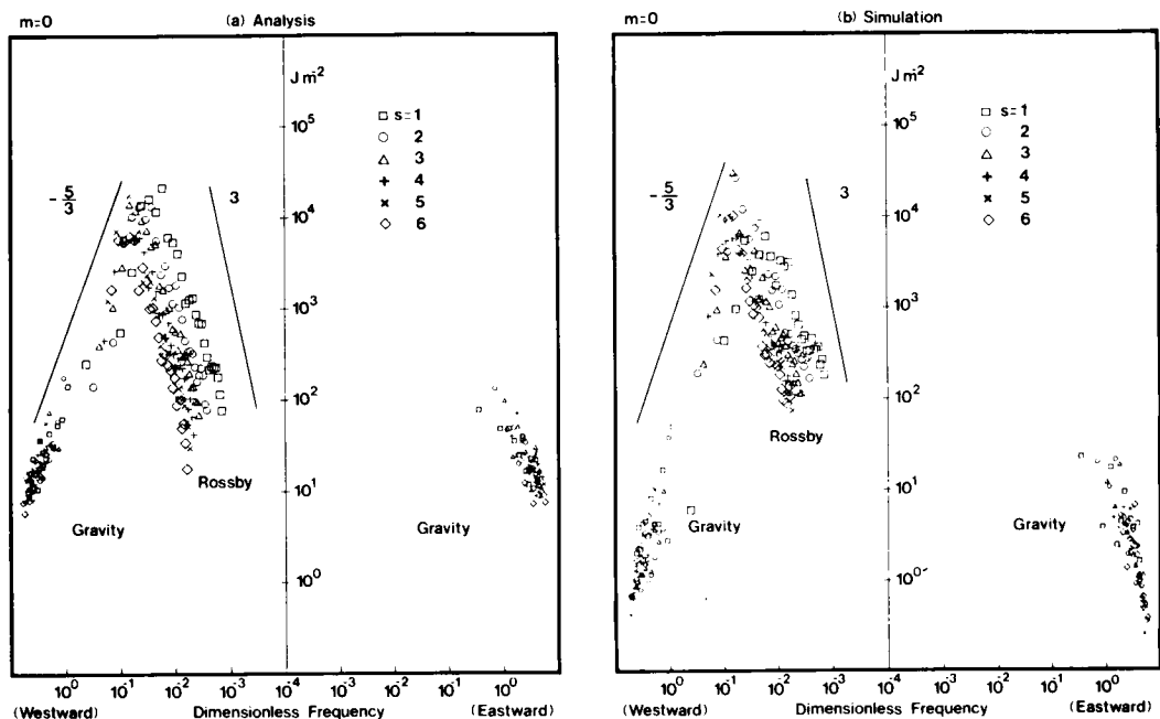
Fig. 6. Distributions of barotropic kinetic energy in the dimensionless frequency domain for (a) GLA analysis and (b) simulation. Large symbols are for the westward propagating Rossby mode and small symbols are for the westward and eastward propagating gravity modes for wavenumbers s=1-6 .
