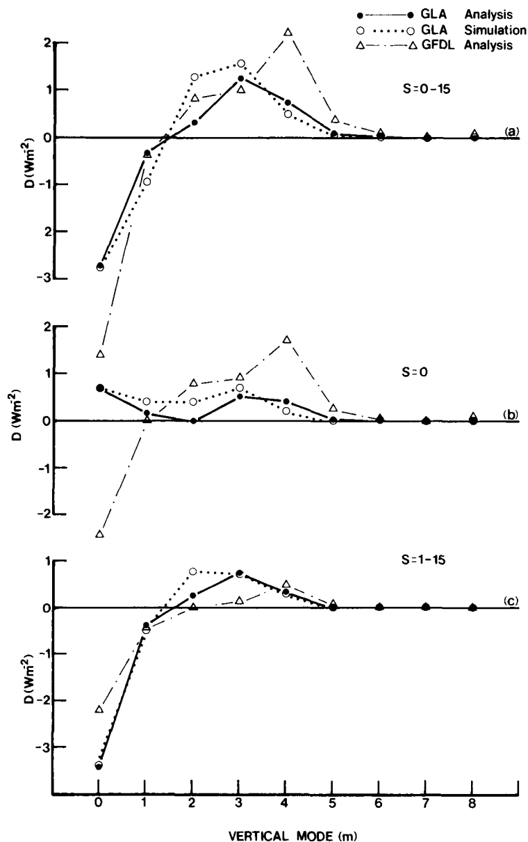
Fig. 9. Rossby mode diabatic process in the vertical mode domain for GLA analysis and simulation and GFDL analysis.
