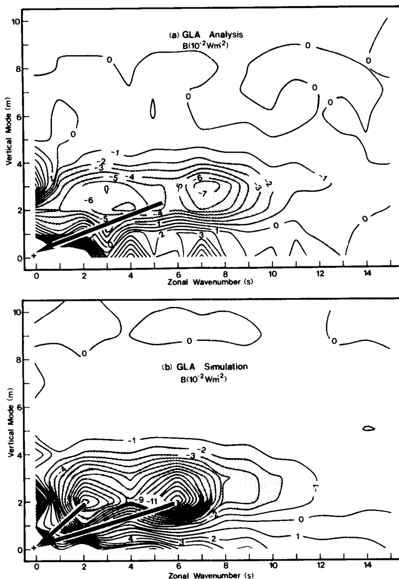
Fig. 8. Interactions of Rossby mode kinetic energy in the wavenumber and vertical mode domains for GLA (a) analysis and (b) simulation in units of 10^{-2} \text{ W m}^{-2} .
