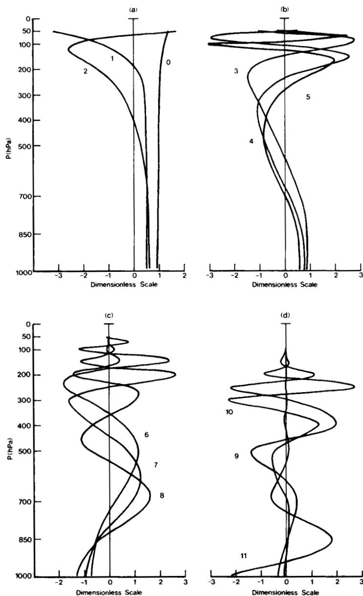
Fig. 1. Vertical eigenvectors for (a) vertical modes m = 0-2 , (b) m = 3-5 , (c) m = 6-8 and (d) m = 9-11 .
