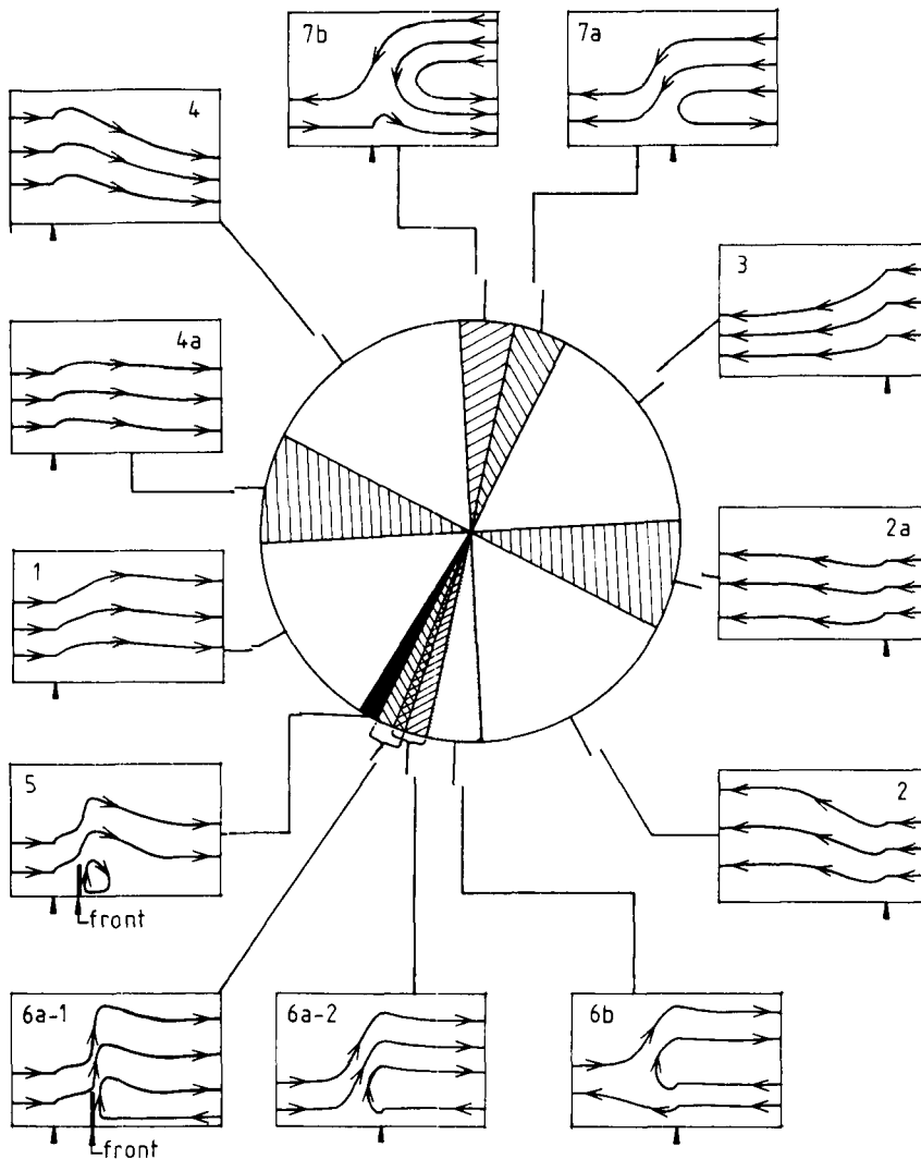
Fig. 3. Overview of the calculated flow regimes, as a function of the geostrophic wind direction. The coast line runs from the top to the bottom of the figure, while the sea is at the left-hand side. The corresponding geostrophic wind vector points from the edge to the centre of the figure. Different shadings correspond to qualitatively different flow patterns; the numbers refer to the discussion in the text. The curves shown in each panel represent trajectory projections on the plane perpendicular to the coastline.
