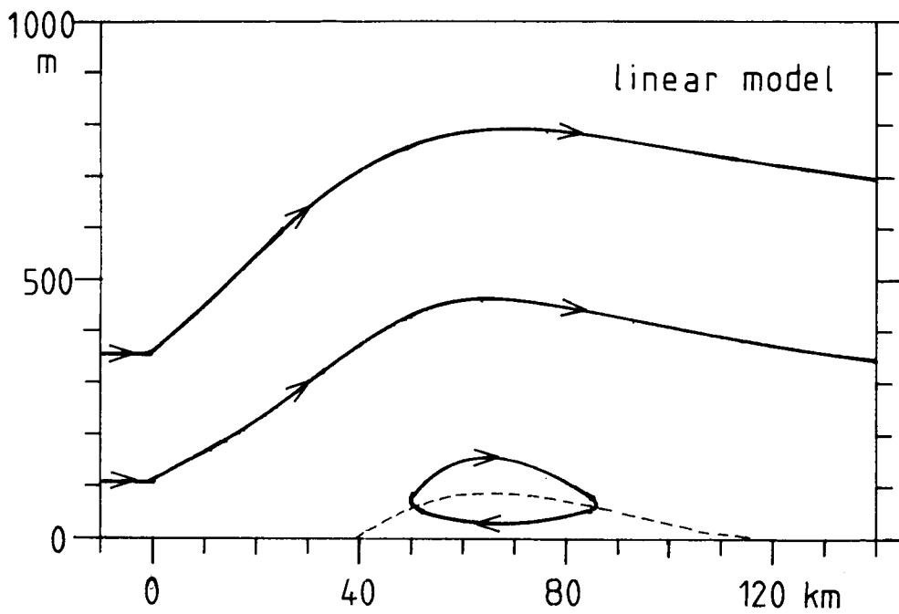
Fig. 6. Comparison between full and linear solution at \phi = 205^\circ . In the area under the broken line, the flow is seaward.
