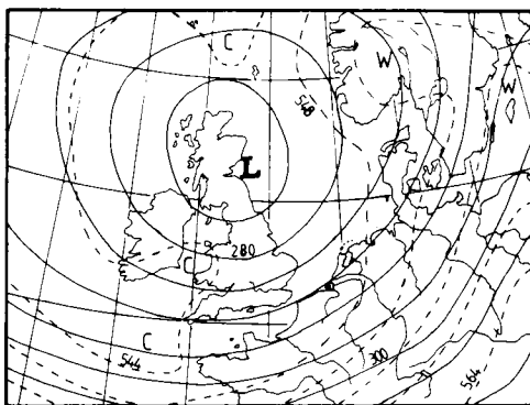
Fig. 7. Map of the 700 mb geopotential height (solid lines) and the 1000/500 mb thickness (dashed lines) at 00 GMT, 16 September 1983. Contour interval: 40 m.
