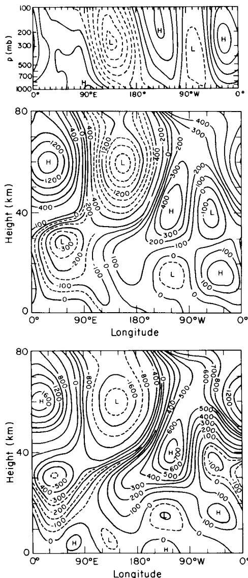
Fig. 13. Longitude-height cross section at 45^\circ\text{N} of stationary-wave geopotential height (a): derived from 11 years of NMC operational analyses by Lau (1979). (The contour interval is 50 m and the zero contour is thickened); (b): calculated for a case corresponding to conditions imposed for Fig. 12c (with U_0 = 3.9 m/s); (c) calculated for a case corresponding to conditions imposed for Fig. 12b (with U_0 = 3 m/s).
