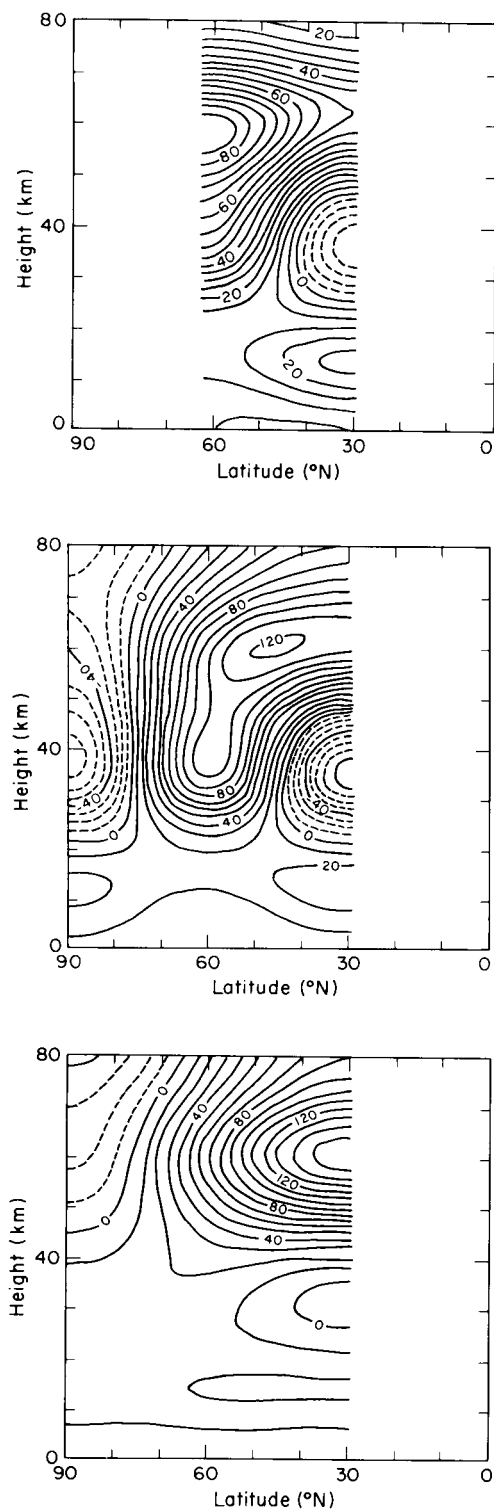
Fig. 12. (a): Distribution of the zonal mean wind \hat{u}(y, z) calculated from the non-linear solution in a 33^\circ channel with \tau_E = 5.7 days and the same \hat{U}_z as used by Tung and Lindzen (1979b), with U_0 = 3.9 m/s. (b): Same as in (a), except for a 60^\circ channel with U_0 = 3 m/s. (c): Same as in (b), except for U_0 = 3.9 m/s.
