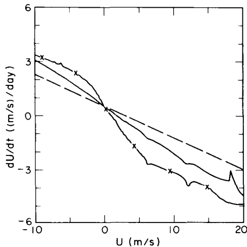
Fig. 14. Phase diagram of dU/dt versus U calculated for \tau_E = 5.7 days, U^* = 3 m/s, a 60^\circ channel, and the same \hat{U}_2 as used by Tung and Lindzen (1979b). The solid curve shows the nonlinear solution and the solid curve marked with crosses shows the linear solution. The dashed straight line shows dU/dt in the absence of mountain torque.
