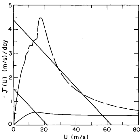
Fig. 9. Mountain torque -J(U) versus U . The notation is the same as in Fig. 5, except now \tau_E = 14.3 days and solutions have been calculated by multiplying the U in the flow over mountain term by the factor \kappa = 0.4 .
