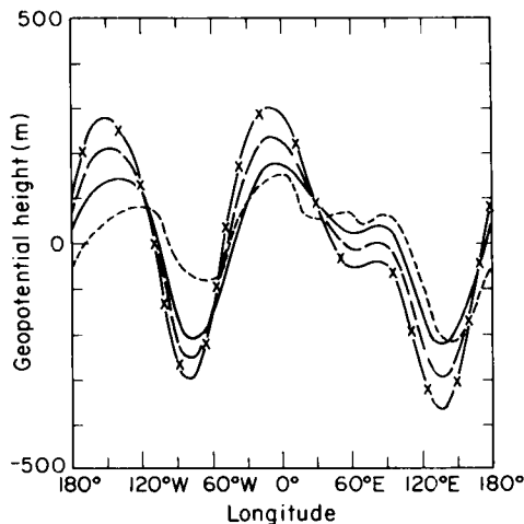
Fig. 11. 500 mb stationary wave geopotential height as a function of longitude at 45^\circ\text{N} when \tau_E = 5.7 days and U = 14 \text{ m/s} . The solid curve shows the nonlinear solution found without transient eddies (but with only topographic forcing); the curve with long dashes is obtained with \chi_{mn} found from the observed amplitude of transient eddy flux (Lau, 1979); and the solid curve marked with crosses is obtained with twice the observed transient heat flux. The curve with short dashes shows the observed winter climatological mean (Oort, 1983).
