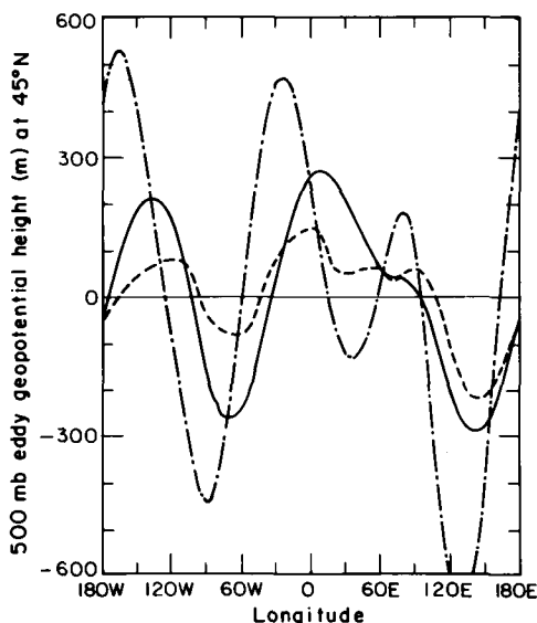
Fig. 8. Same as in Fig. 7 except for \tau_E = 14.3 days.
