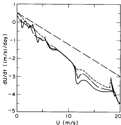
Fig. 16. Phase diagram of dU/dt versus U . The curve with short dashes shows the nonlinear solution for the same case as in Fig. 14 (without transient eddy heat fluxes); the curve with long dashes shows the solution when \chi_{mn} has values inferred from the observed climatological transient eddy heat flux (Lau, 1979); and the solid curve shows the solution calculated using twice these values. U^* = 3 m/s. The abscissa should be shifted for other values of U^* .
