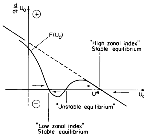
Fig. 1. A schematic phase diagram of dU_0/dt = F(U_0) versus U_0 for the case when the mountain torque creates a large deceleration of the zonal index on the low side of U^* . The dashed straight line is F(U_0) in the absence of mountain torque. One stable equilibrium exists at U_0 = U^* for the no-mountain case, and three equilibrium points (two stable and one unstable) appear in the case with mountains. Arrows indicate the direction that U_0 tends.
