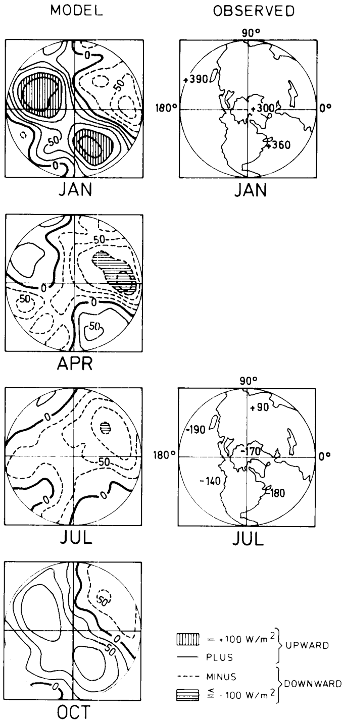
Fig. 9. Net heat flux north of 12.5^\circ\text{N} . Left-hand side: inferred from model regression analysis; right-hand side: observations, from Schutz and Gates (1971, 1972).
