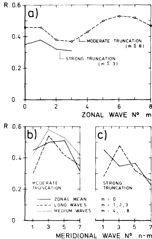
Fig. 5. Change-of-state correlation for \tau = 6 days as a function of zonal and meridional wavenumbers. Panel (a) refers to the superposition of all 4 meridional wave-numbers, panels (b) and (c) to the separate superposition patterns for medium-, long-wave and zonal mean components. Both moderately and strongly truncated models are shown.
