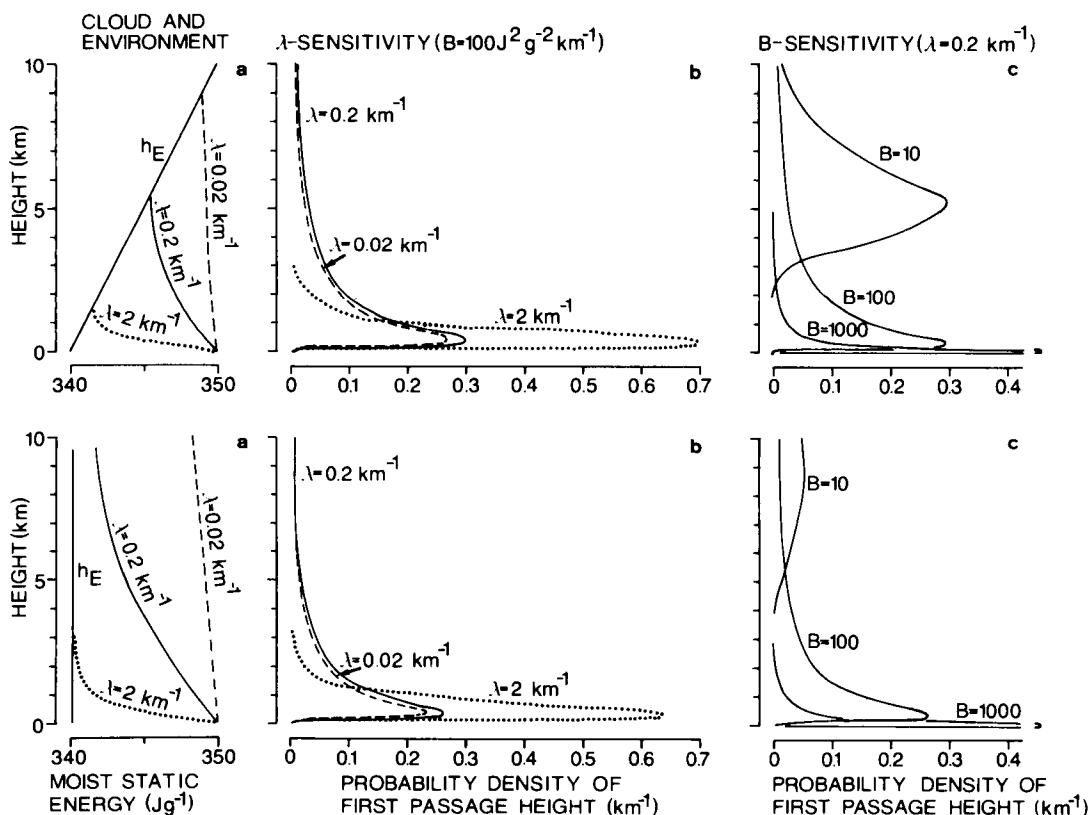
Fig. 3. Same as Fig. 1 except for a linearly increasing h_e profile (top) and h_e constant (bottom).
