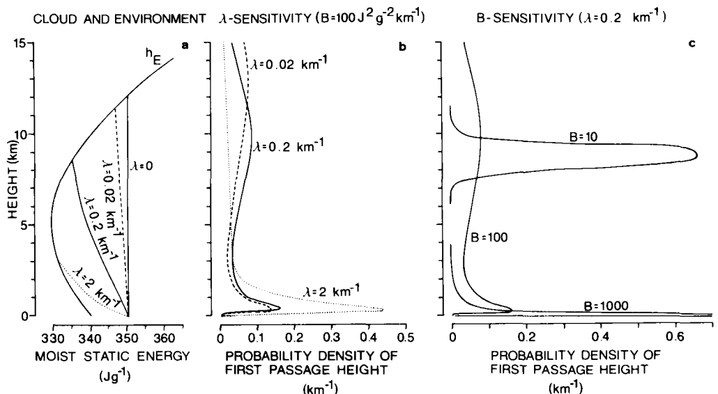
Fig. 1. (a) Moist static energy of clouds with varying entrainment rates in a tropical environment h_e (above cloud base). Probability densities of first passage or cloud top heights depending on (b) the entrainment rate ( \lambda -sensitivity) and (c) on the intensity of the stochastic fluctuations ( B -sensitivity).
