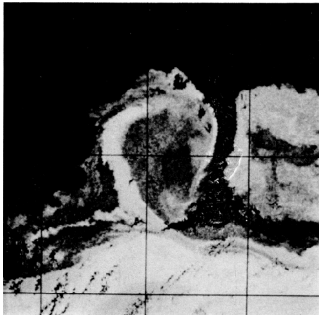
Fig. 4. Atmospherically corrected NOAA-7 AVHRR infrared image of a typical warm-core ring (courtesy of O. Brown and R. Evans). Note that the ring's shape is similar to an ellipse oriented in the N-S direction as predicted by the model. The ring is centered at approximately 40^\circ\text{N} and 64^\circ\text{W} . The grid is 2^\circ \times 2^\circ latitude longitude on a navigated image remapped to a mercator projection. Image was processed by the University of Miami, Remote Sensing Center.
