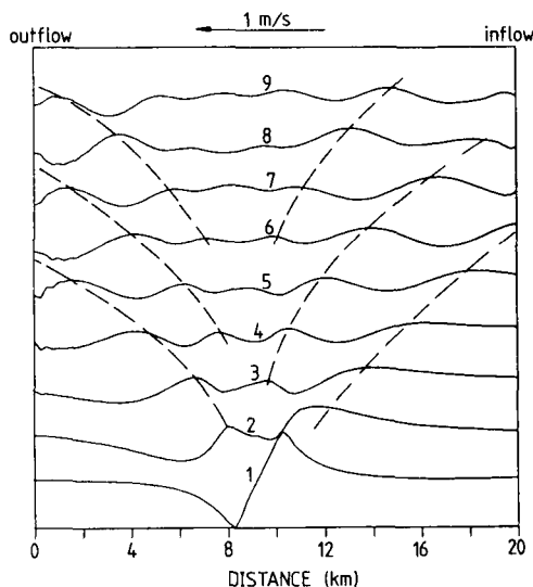
Fig. 2. A test run on a small domain in which gravity waves are generated by switching on a local heat source for a short time. Solid lines show the stream function at a height of 1000 m. Time interval between curves is 5 min. Vertical velocities associated with these gravity waves are typically 10 \text{ cm s}^{-1} .
