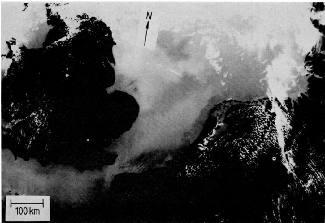
Fig. 1. IR-image from TIROS-N (22 July, 1983; 14:36 GMT), showing enhanced cumulus convection along a sea-breeze front in the western part of the Netherlands. Reproduced with permission of the University of Dundee.
