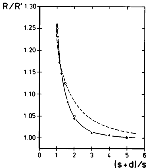
Fig. 1. Ratio of the reflection R from an array of cubic clouds to the reflection R' from an isolated cloud at a single wavelength ( \lambda = 450 nm). \circ Aida (1977). --- Harshvardhan and Weinman (1982b). — + this work. s is the cloud dimension and d the separation of individual cloud. Single-scattering albedo: \bar{\omega} = 0.9999 ; optical depth: \tau = 49 ; zenith angle: \theta_0 = 0^\circ .
