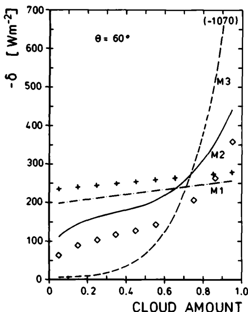
Fig. 10. Net radiative effect \delta (see eq. (1)) as a function of cloud amount (note that \delta is negative) for 3 cloud models (M1: dash-dotted; M2: solid; M3: dashed line). Cloud and atmosphere are as in Fig. 8 and the solar zenith angle is \theta = 60^\circ . Crosses (+) denote results of a run using the M1 cloud but neglecting atmospheric aerosol. Diamonds (◇) show results for an M2 run, increasing the surface albedo from 0.1 to 0.3.
