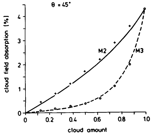
Fig. 7. Cloud field absorption versus cloud amount. Comparison between exact Monte Carlo results and the parameterization using the effective cloud cover for solar reflection. Solar zenith angle is \theta = 45^\circ . M2 and M3 are different cloud models.
