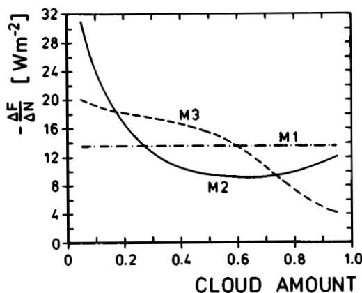
Fig. 9. Change of the outgoing long-wave flux F with cloud amount versus cloud amount for 3 cloud models M1, M2 and M3 (note that \partial F/\partial N is negative). Cloud and atmosphere are as in Fig. 8.
