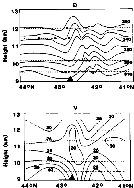
Fig. 9. Cross section of potential temperatures in K along a north-south line between 44°N and 41°N for March 23, 1982 using a combination of all FALCON legs. Dashed lines indicate the flight legs. The bottom figure shows the corresponding meridional wind field. Note that v greater than zero represents winds from the north and that just the upper part of the atmosphere from 9 to 13 km is shown. The crosses mark regions, where light to moderate turbulence was encountered.
