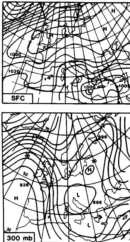
Fig. 1. Surface pressure chart (top) and 300 mb chart (bottom) for March 23, 1982. The increment of pressure in the surface chart is 5 mb. The increment at 300 mb is 8 gpm.
