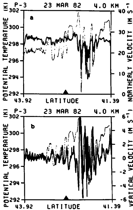
Fig. 11. Potential temperature (thin), northerly winds ((a), solid) and vertical velocity ((b), solid) from the P-3 flight record at the 4.0 km level. The mountain crest is indicated by the black triangle.
