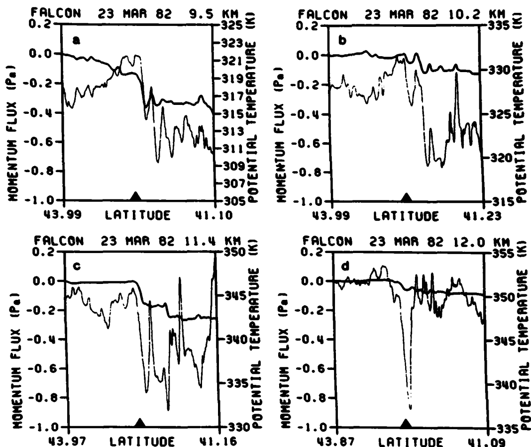
Fig. 19. As in Fig. 17 except for the FALCON flight legs at 9.5 km (a), 10.2 km (b), 11.4 km (c) and 12.0 km (d).
