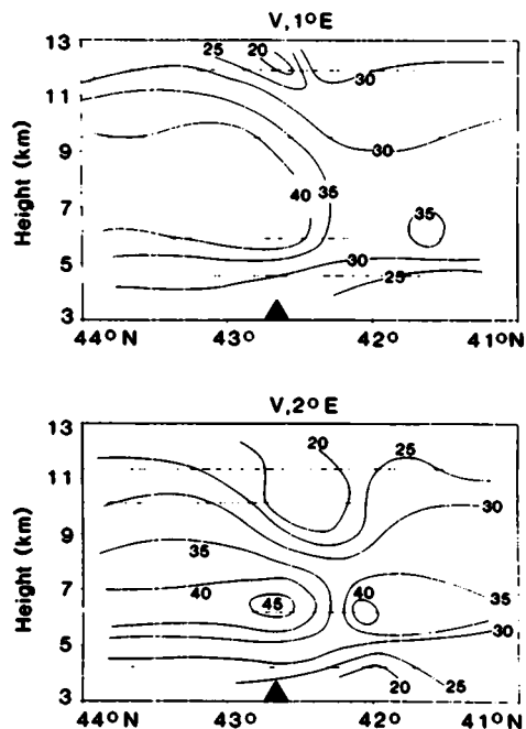
Fig. 7. As in Fig. 6, except for the northerly wind component in \text{ms}^{-1} . Note, that v greater than zero represents winds from north.
