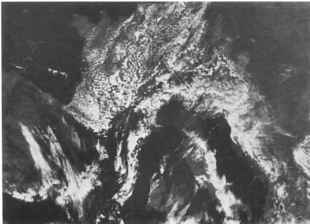
Fig. 2. Satellite picture (NOAA 7, AVHRR channel 2) at March 23, 1982 1320 GMT. Spain is located at the left-hand edge.
