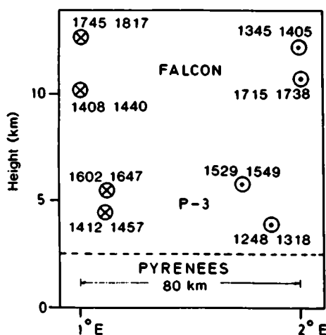
Fig. 4. West-east cross section above the Pyrenees showing schematically the flight patterns of the DFVLR-aircraft FALCON and the NOAA-aircraft P-3. The crosses indicate northerly flight tracks while dots stand for southerly tracks. Note the times in GMT of the start and end of the cross flights. The abscissa is given in degrees of longitude.
