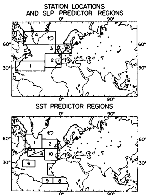
Fig. 1. Location of surface air temperature stations (solid dots) used in this study. Also shown on the upper and lower panels, respectively, are the predictor averaging areas for sea level pressure (SLP) and sea surface temperature (SST).
