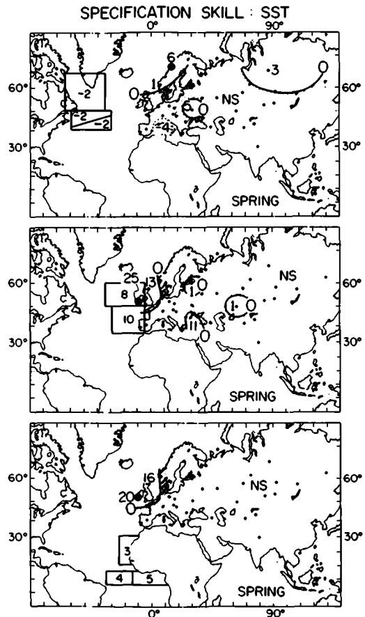
Fig. 3. The ability of SST in selected Atlantic regions to specify subsequent air temperature anomalies over Eurasia. A significant model could not be constructed for the regions denoted by "NS". Specification skill at the few significant stations shown in this illustration rarely exceeded 5%. The prediction coefficient (eq. 3), multiplied by 100, is shown in the appropriate predictor region (small numbers in the boxes) for Bodö (top) and Valentia (middle and bottom). These stations are denoted by an oversized station dot.
