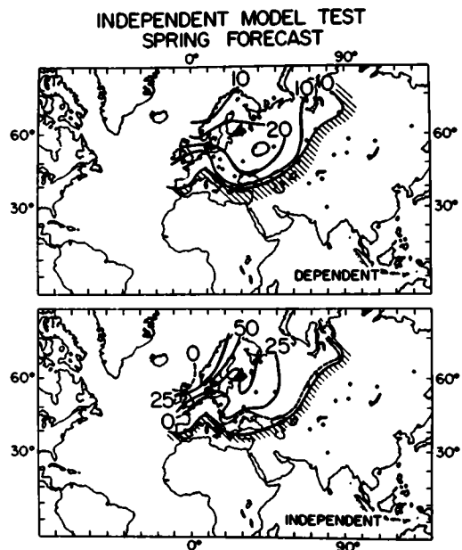
Fig. 9. Forecast experiment on independent data. The upper panel shows the hindcast skill (percent of variance) associated with the dependent model construction for the period 1902–1971. The lower panel shows the forecast skill over the 1972–1978 period. The heavy dashed line represents the "zero skill" line associated with the independent test. Note that over most of the region it follows the zero line derived from the dependent test.
